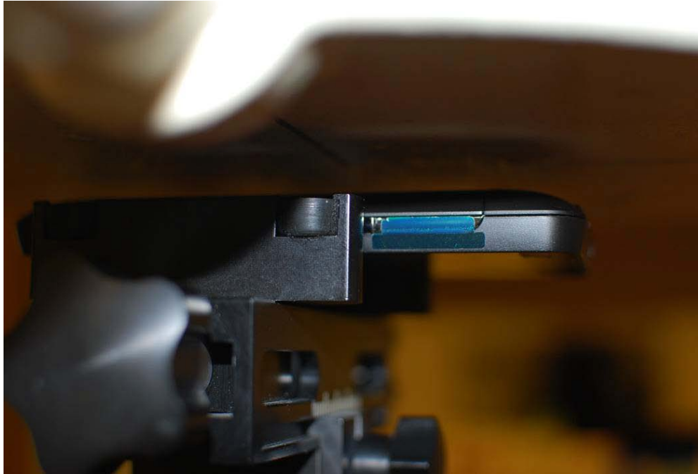
Figure 22-5 SAR Test Setup Photo 6: Back Side
