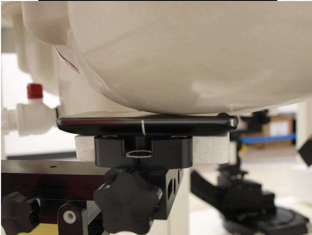
LEFT HAND SIDE TOUCH (with wireless charger back cover)
