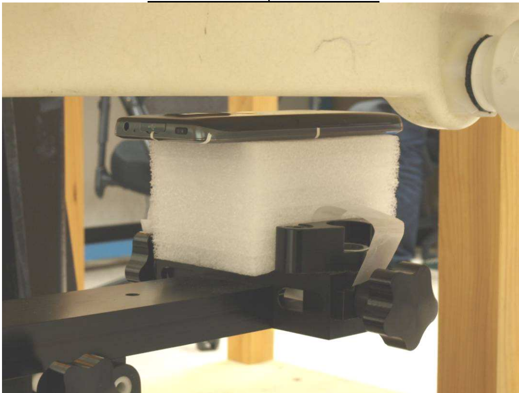
Body & Hotspot Rear w/ 10 mm separation distance
