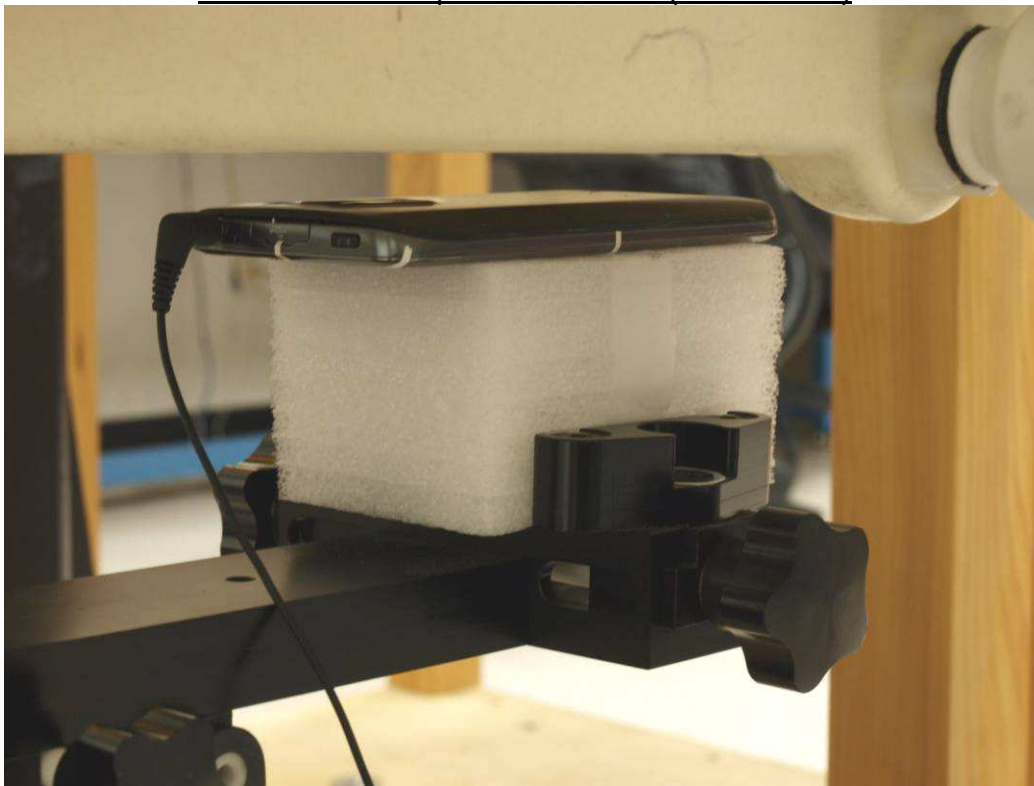
Body & Hotspot Rear w/ 10 mm separation distance (with headset)
