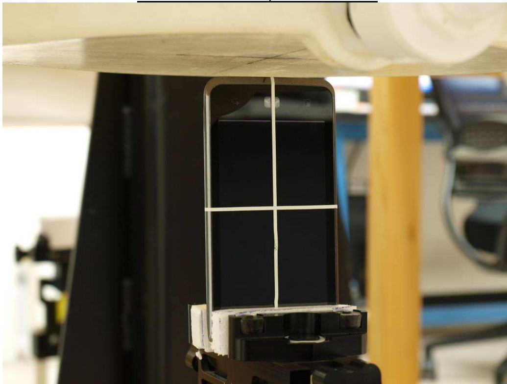
Body & Hotspot Bottom w/ 10 mm separation distance
