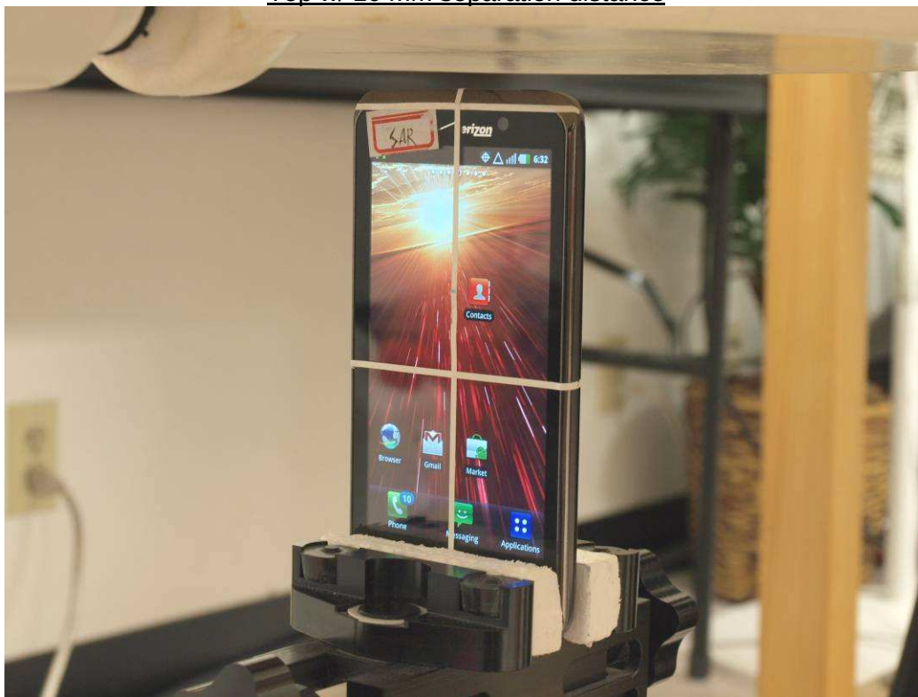
Body & Hotspot Top w/ 10 mm separation distance
