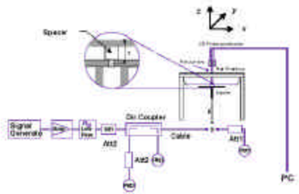
Figure 12.1 Dipole Validati
