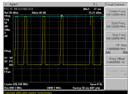
Figure 26 Zero-Span Plots and Channel power correlation
