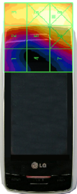
Figure 17-4 E-Field WD Scan overlay
