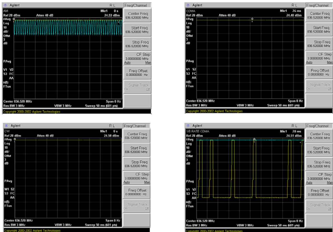
Figure 23 Zero-Span Plots
