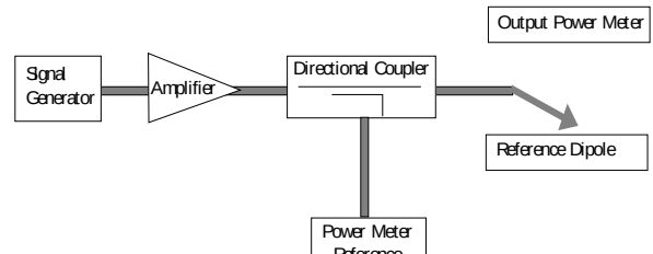
Figure 14 Setup to Dipole
