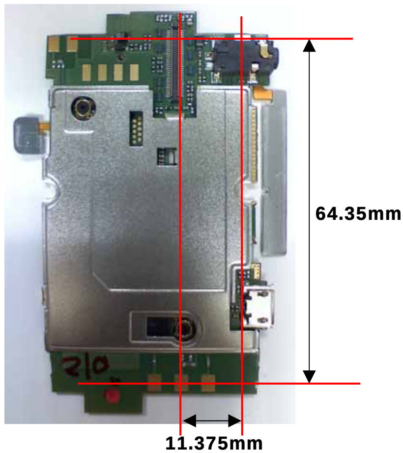
- . Feeding distance between antennas
