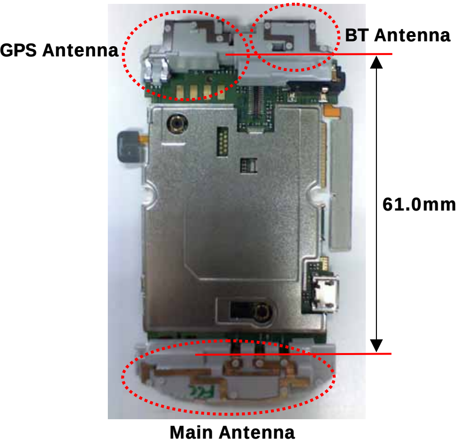
- . Pattern distance between antennas
