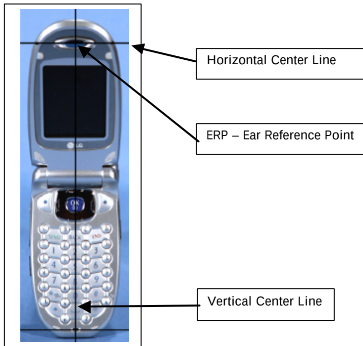
Figure 13.1 Handset Reference Points
