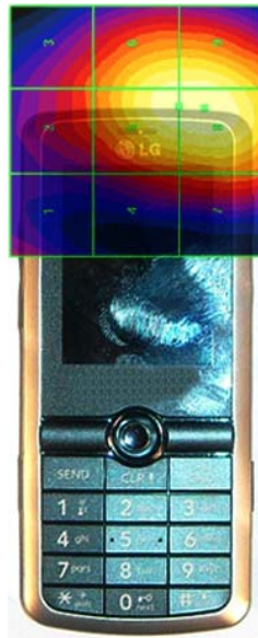
Figure 17-4 E-Field WD Scan overlay
