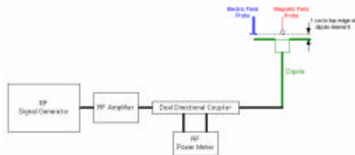
Figure 21 System Check Setup
