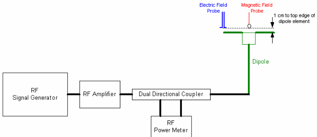
Figure 25 Determining Modulation Factor Probe Setup
