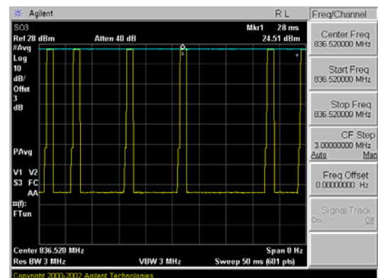
Figure 23 Zero-Span Plots
