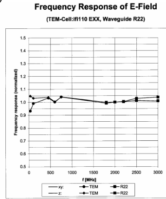
Figure 5 E-Field Probe Frequency Response
