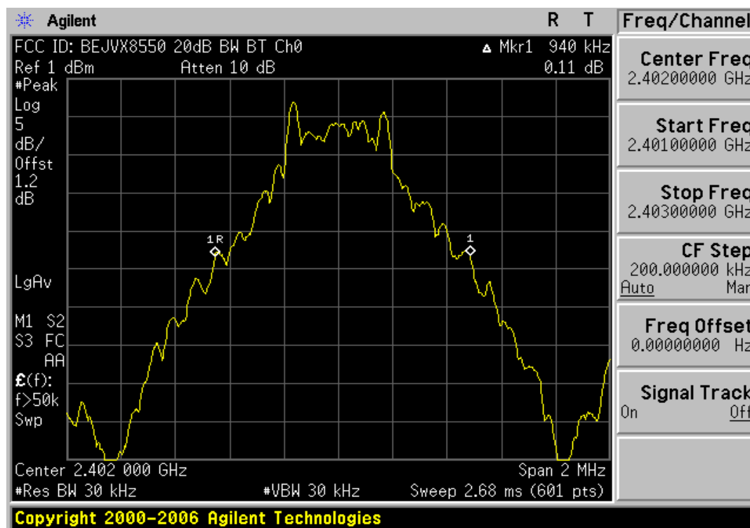
Plot 6-1. 20dB Bandwidth Plot (Bluetooth – Ch. 0)
