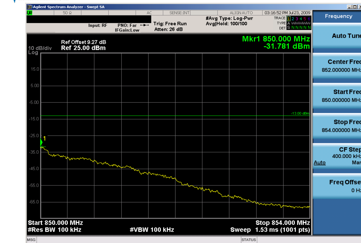
Plot 7-11. 4MHz Span Plot (Cellular CDMA Mode – Ch. 777)
