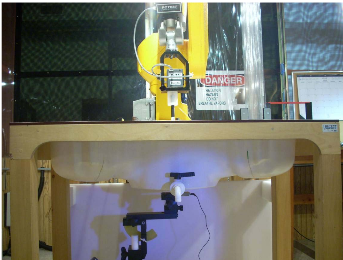
Figure 7: Body SAR
