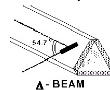
Figure 4-2 Probe Thick Film Technique
