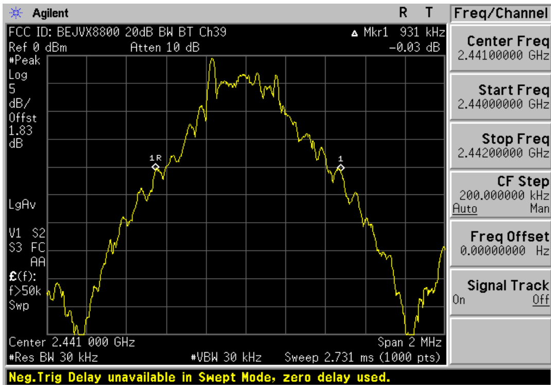
Plot 6-2. 20dB Bandwidth Plot (Bluetooth – Ch. 39)
