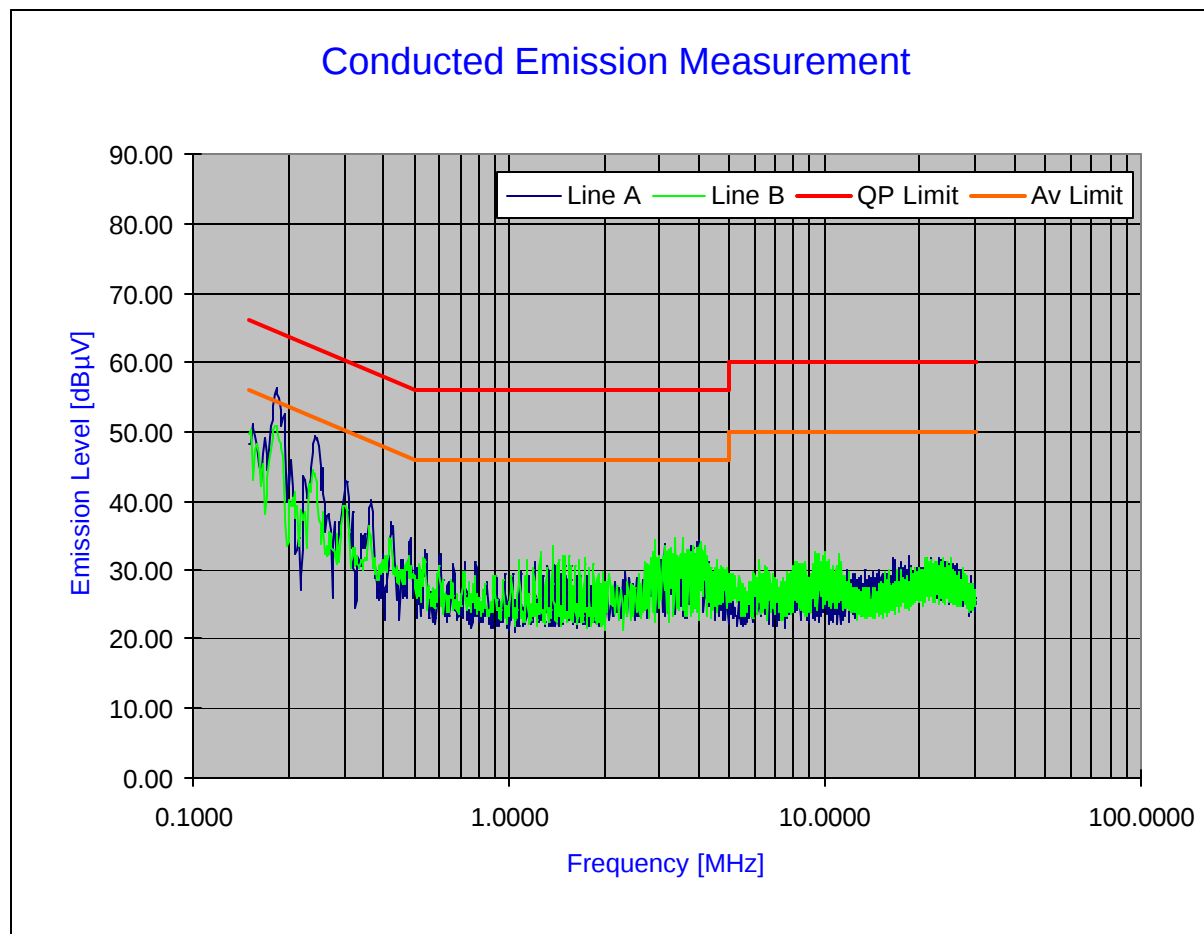
Plot 7-1. Line-Conducted Test Plot
