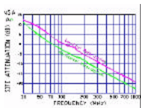
Figure 3-8. Normalized Site Attenuation Curves (H&V)
