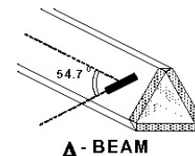
Figure 4-3 Triangular Probe Configuration
