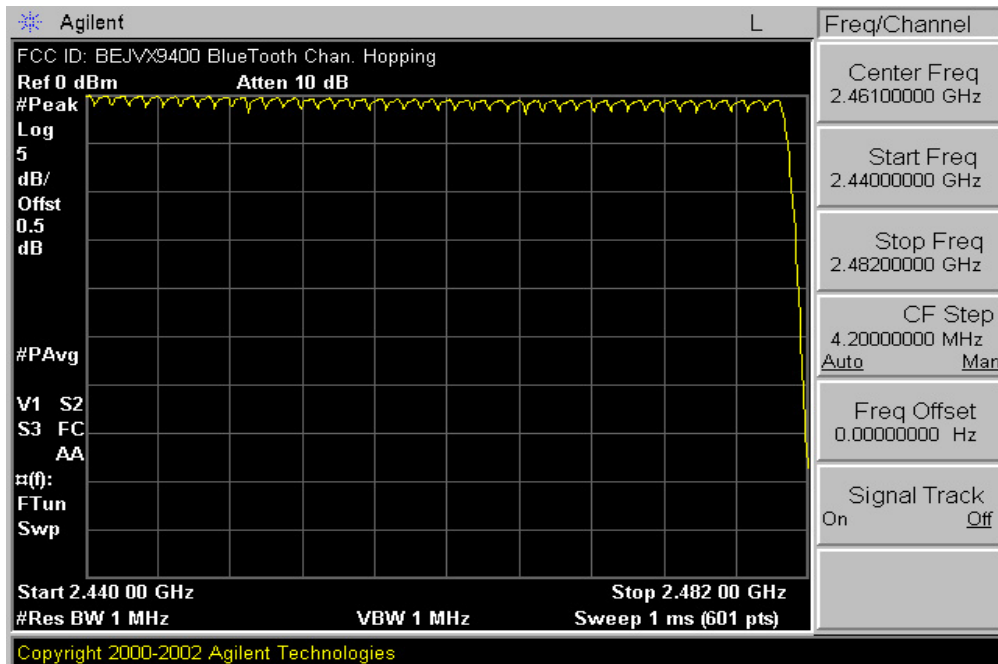
Plot 6-9. High End Spectrum Channel Hopping Plot (Bluetooth)
