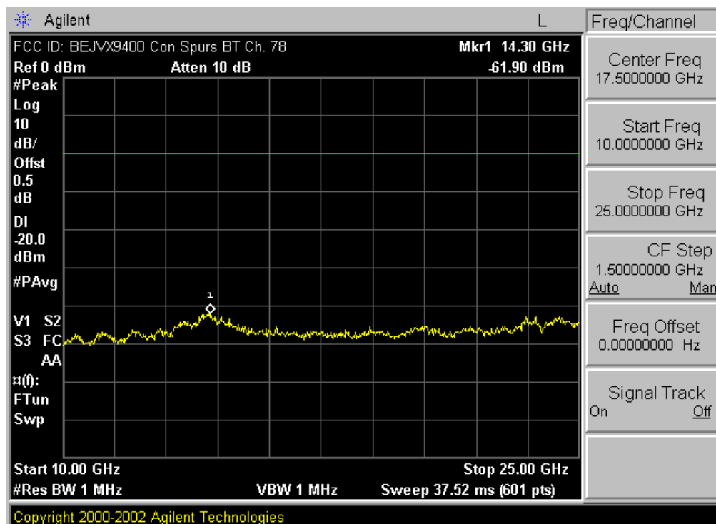
Plot 6-15. Conducted Spurious Plot (Bluetooth – Ch. 78)
