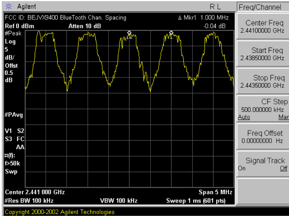
Plot 6-6. Channel Spacing Plot (Bluetooth)
