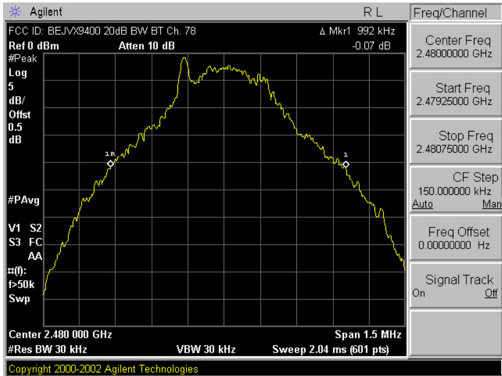
Plot 6-3. 20dB Bandwidth Plot (Bluetooth – Ch. 78)
