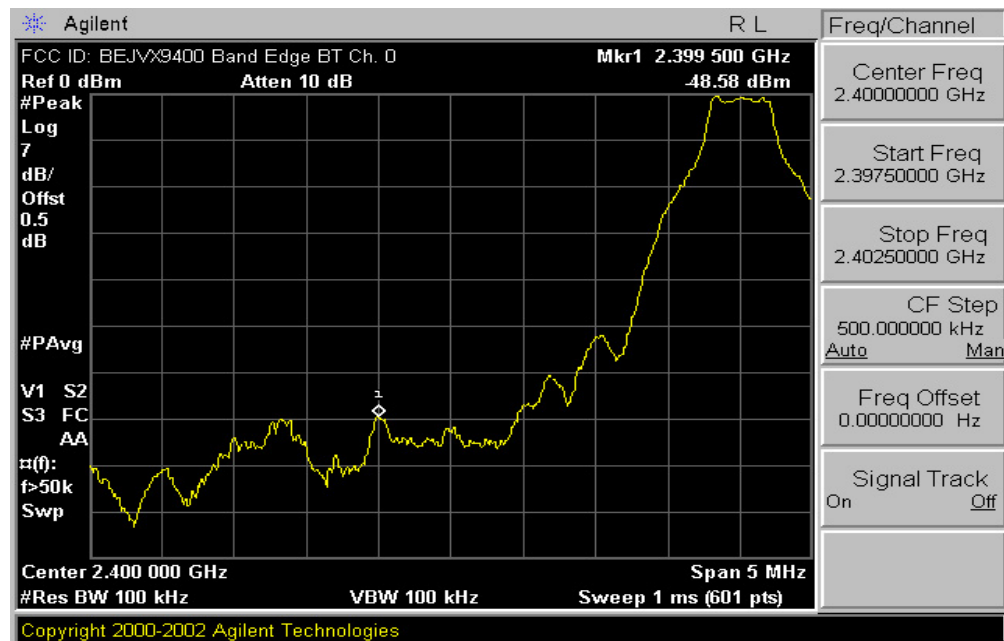
Plot 6-4. Band Edge Plot (Bluetooth – Ch. 0)
