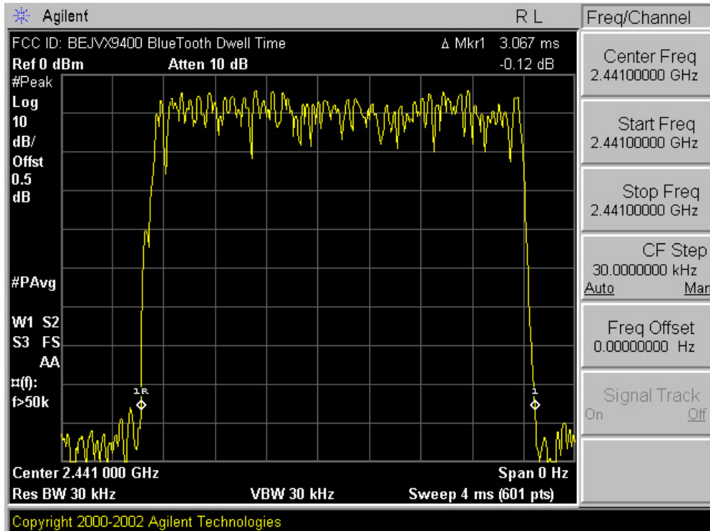
Plot 6-7. Time of Occupancy Plot (Bluetooth)
