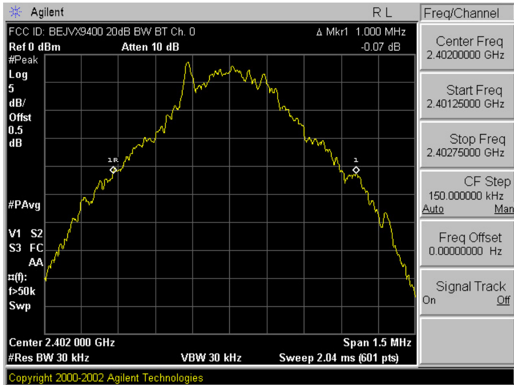
Plot 6-1. 20dB Bandwidth Plot (Bluetooth – Ch. 0)
