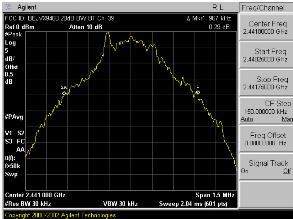
Plot 6-2. 20dB Bandwidth Plot (Bluetooth – Ch. 39)
