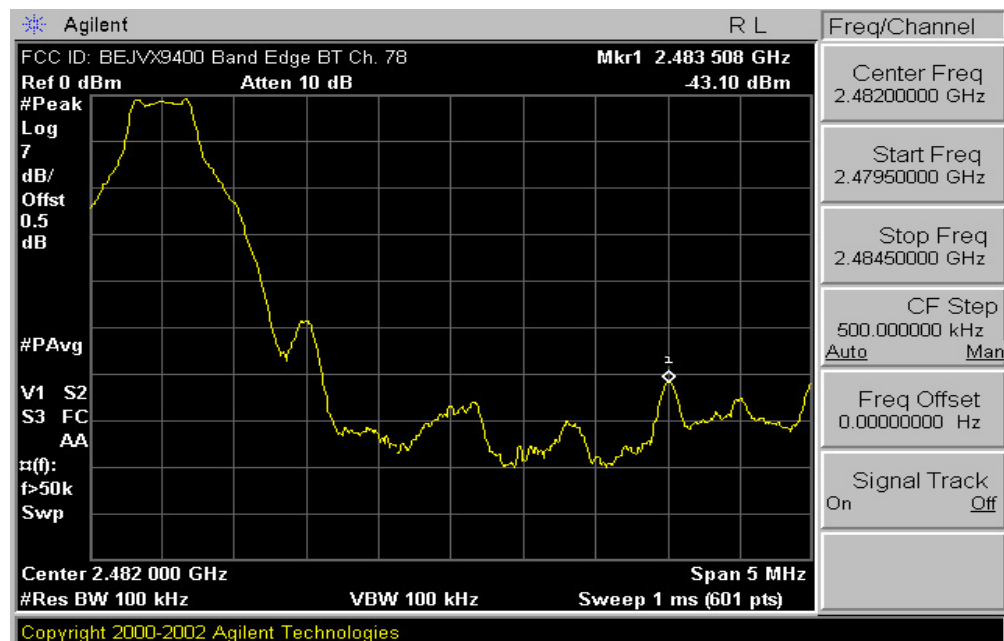
Plot 6-5. Band Edge Plot (Bluetooth – Ch. 78)
