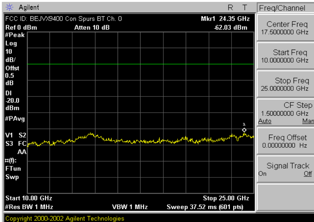
Plot 6-11. Conducted Spurious Plot (Bluetooth – Ch. 0)
