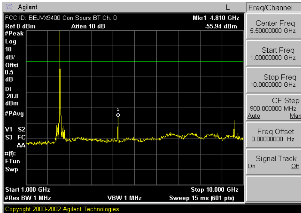
Plot 6-10. Conducted Spurious Plot (Bluetooth – Ch. 0)
