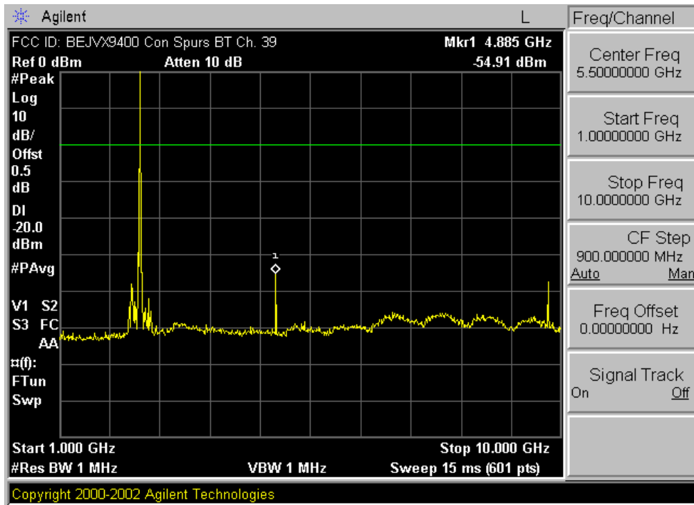
Plot 6-12. Conducted Spurious Plot (Bluetooth – Ch. 39)
