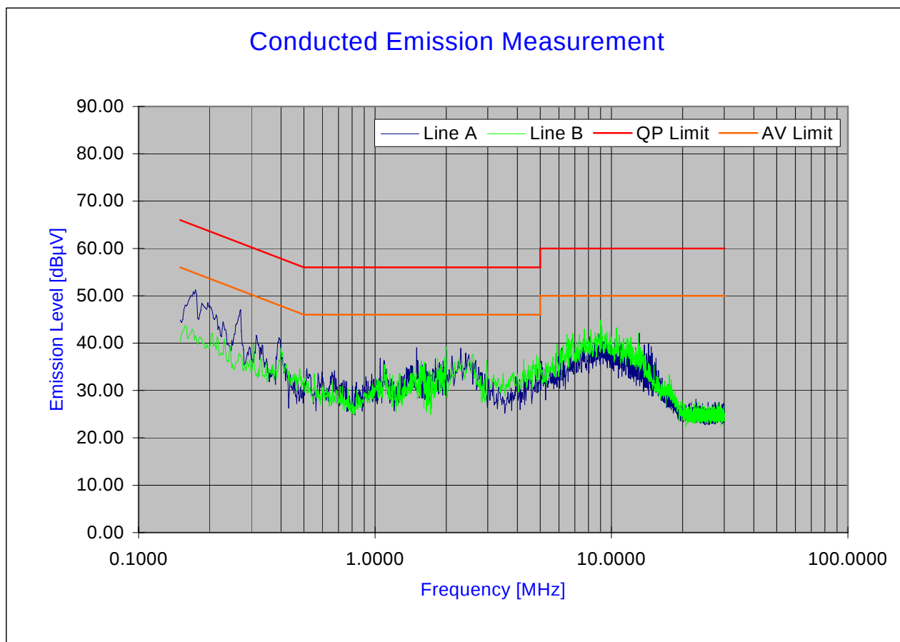
Plot C-1. Line-Conducted Test Plot
