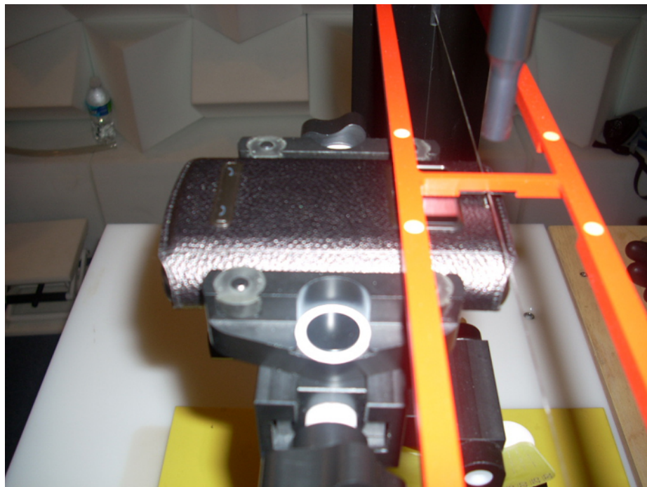
Figure 17-4 HAC Phantom Plane Alignment with Leather Case
