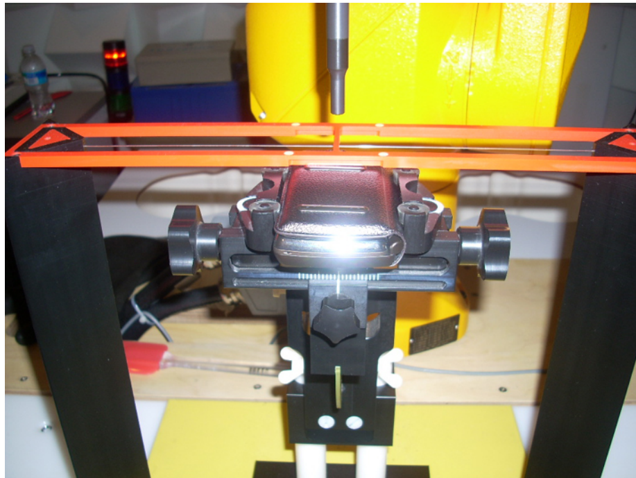
Figure 17-3 Ear Reference Point HAC Phantom Alignment with Leather Case
