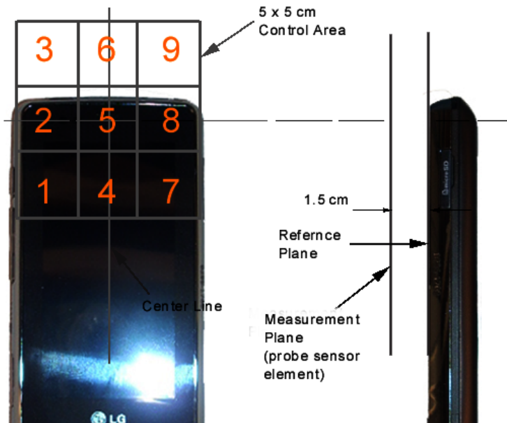
Figure 17-5 5x5 Scan grid above WD
