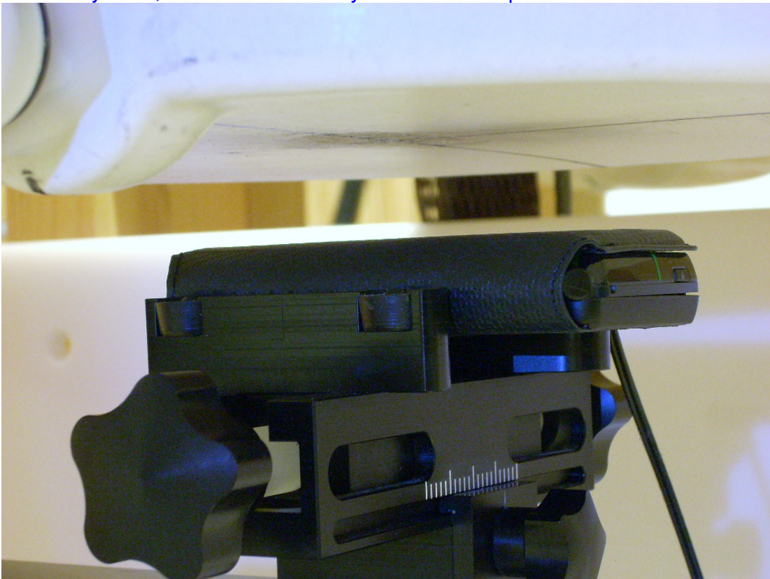
12. Body SAR, Front Side with Keyboard 20mm Space
