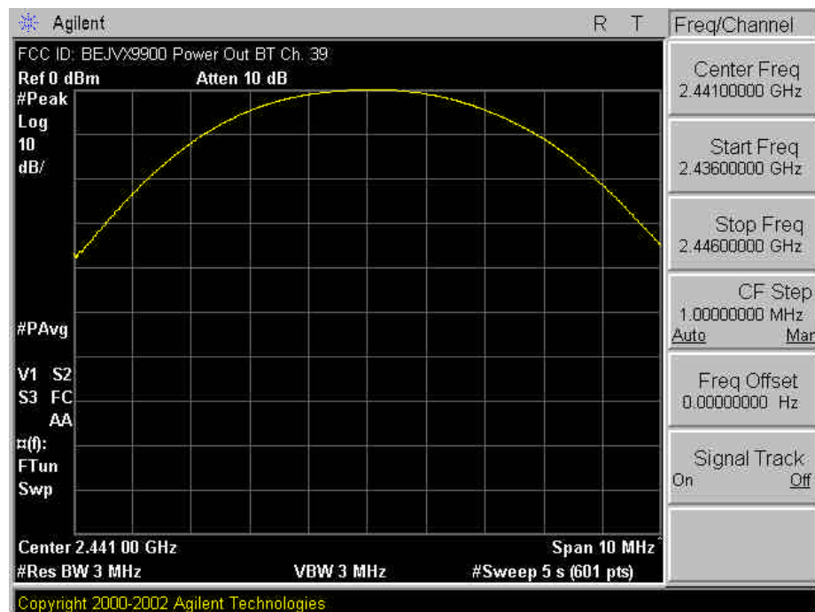
Plot A-5. Max. Peak Output Power Plot – Ch. 39
