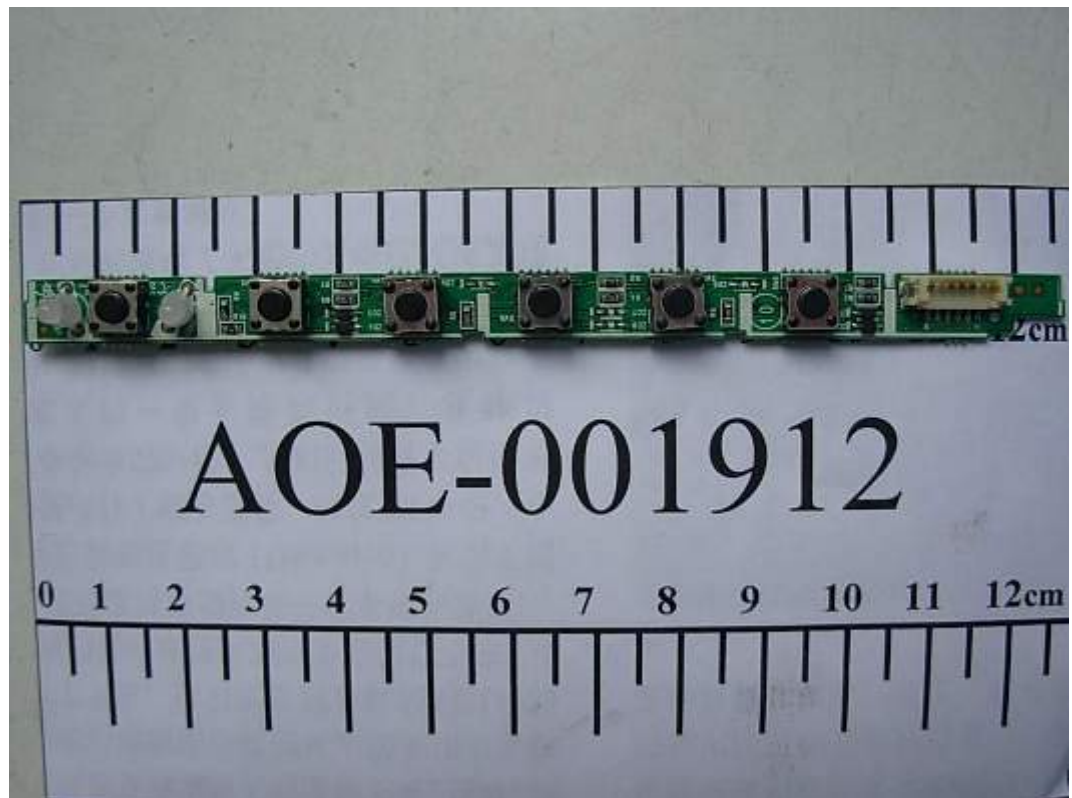
FIGURE 2 LCD MONITOR (M/N: W1542ST) KEY BOARD (COMPONENT SIDE)
