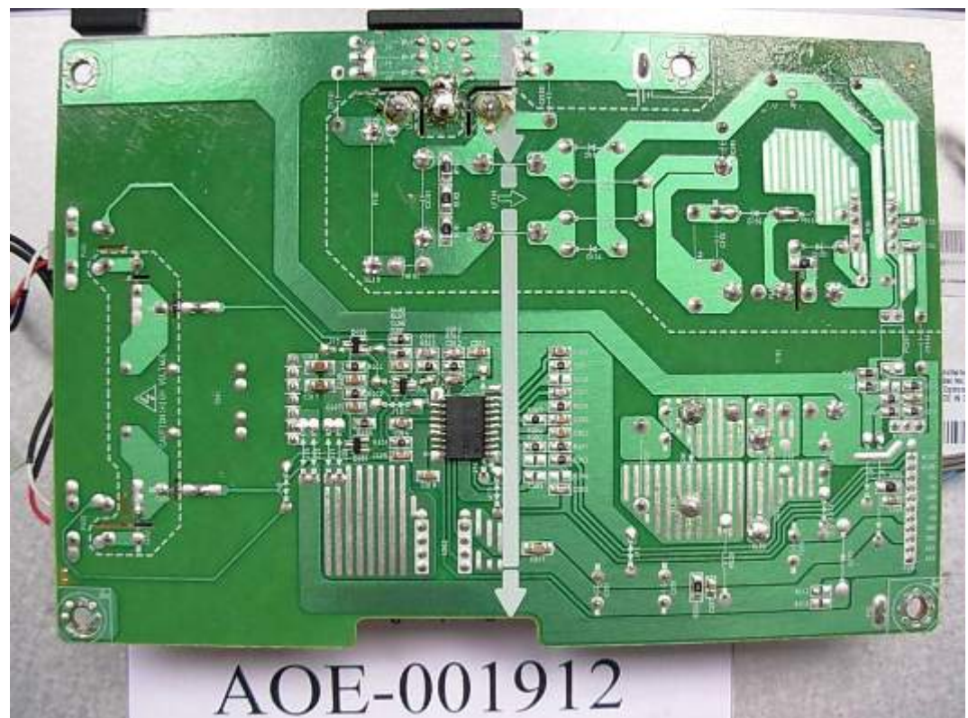
FIGURE 10 LCD MONITOR (M/N: W1542ST) POWER BOARD (SOLDERED SIDE)
