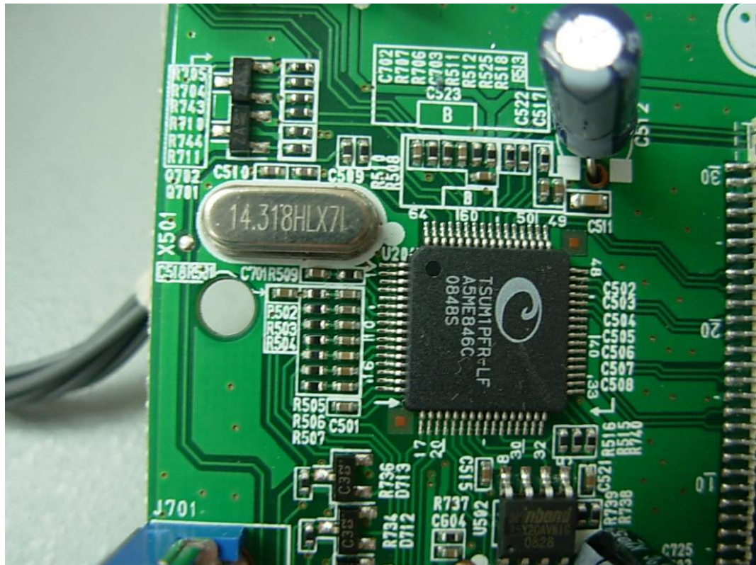
FIGURE 9 LCD MONITOR (M/N: W1642CT) CHIP & CRYSTAL ON MAIN BOARD
