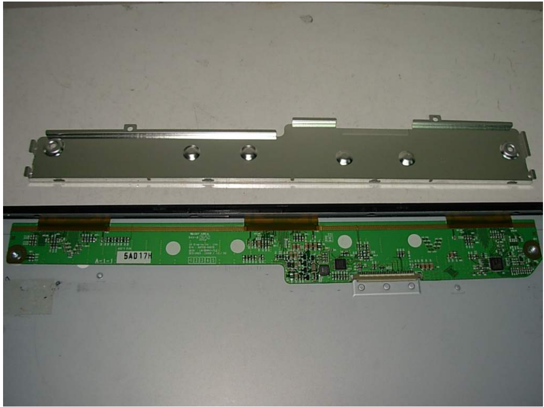
FIGURE 11 LCD MONITOR (M/N: W1642CT) LCD PANEL MAIN BOARD SHIELDED SHELL REMOVED
