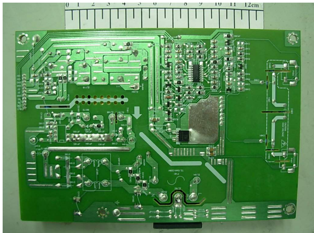
FIGURE 6 LCD MONITOR (M/N: W1642CT) POWER BOARD (SOLDERED SIDE)
