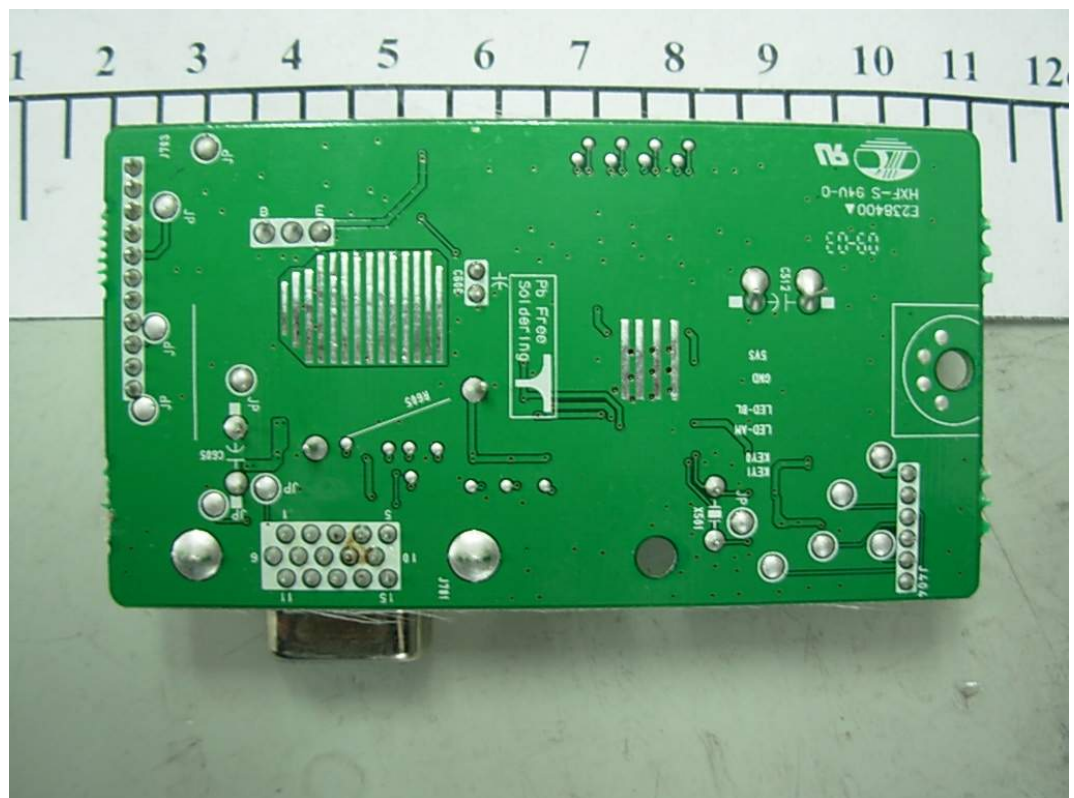
FIGURE 8 LCD MONITOR (M/N: W1642CT) MAIN BOARD (SOLDERED SIDE)
