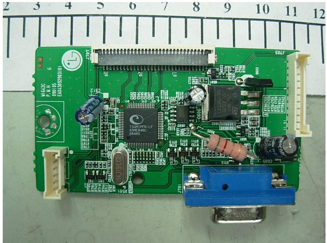
FIGURE 7 LCD MONITOR (M/N: W1642CT) MAIN BOARD (COMPONENT SIDE)
