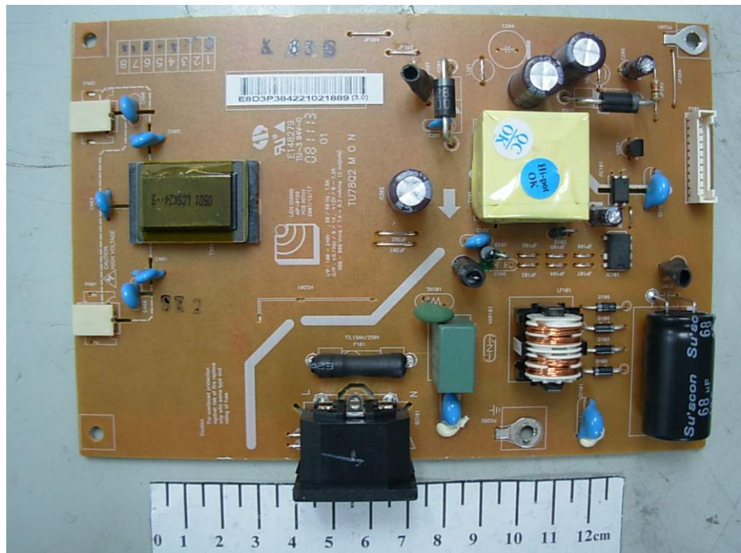
FIGURE 5 LCD MONITOR (M/N: W1642CT) POWER BOARD (COMPONENT SIDE)
