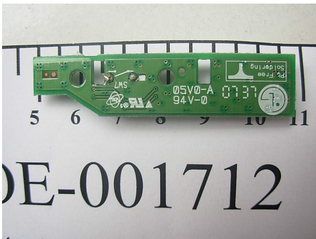
FIGURE 5 LCD MONITOR (M/N: W1752ST) LED BOARD (BACK VIEW)
