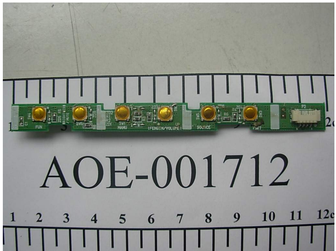
FIGURE 2 LCD MONITOR (M/N: W1752ST) BUTTON BOARD (FRONT VIEW)
