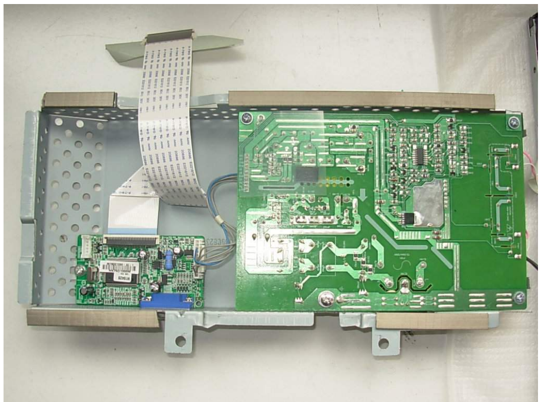
FIGURE 19 LCD MONITOR (M/N: W1752ST) DEBUG
