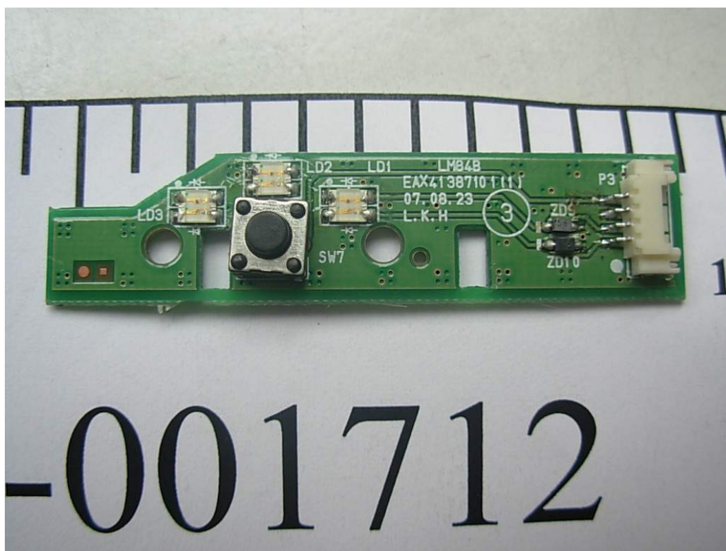
FIGURE 4 LCD MONITOR (M/N: W1752ST) LED BOARD (FRONT VIEW)
