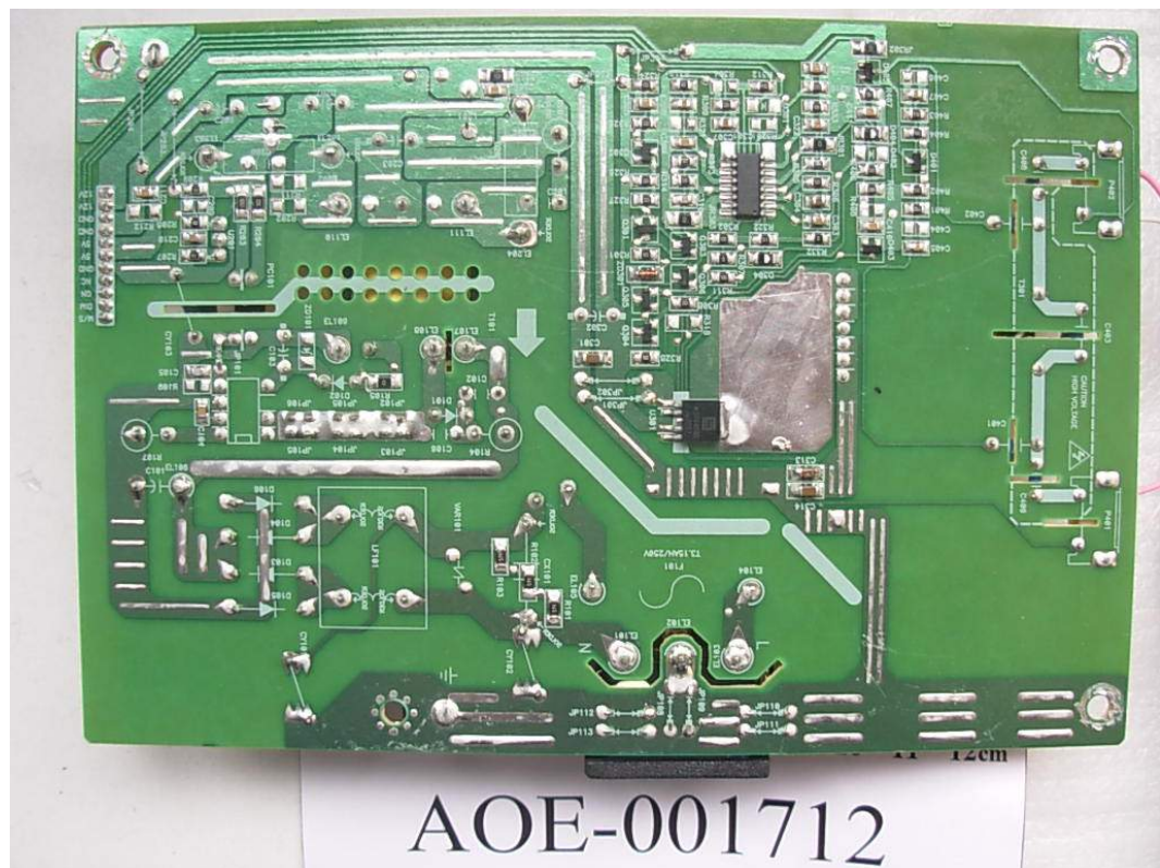
FIGURE 12 LCD MONITOR (M/N: W1752ST) POWER BOARD (BACK VIEW)
