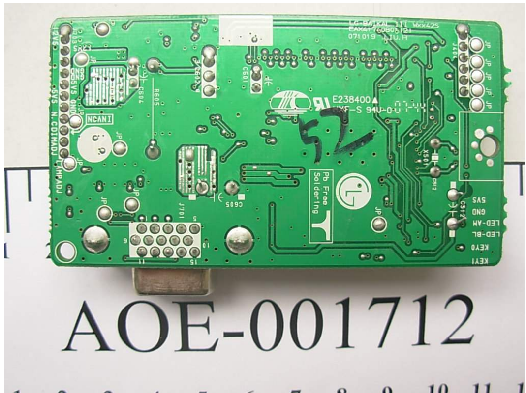
FIGURE 8 LCD MONITOR (M/N: W1752ST) MAIN BOARD (SOLDERED SIDE)
