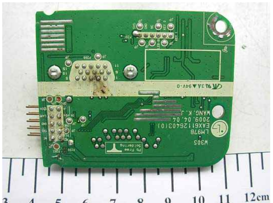
FIGURE 8 LCD MONITOR (M/N: W1930SV) MAIN BOARD (SOLDERED SIDE)
