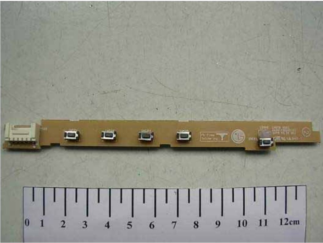
FIGURE 3 LCD MONITOR (M/N: W1930SV) KEY BOARD (COMPONENT SIDE)
