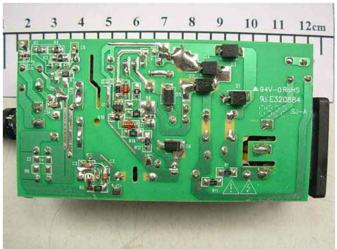
FIGURE 31 LCD MONITOR (M/N: W1930SV) ADAPTER #3 MAIN BOARD (SOLDERED SIDE)
