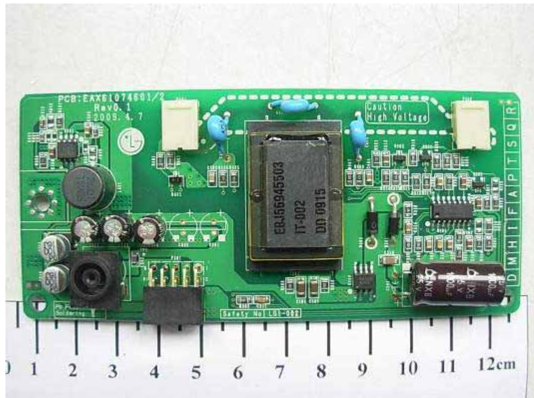
FIGURE 5 LCD MONITOR (M/N: W1930SV) POWER BOARD (COMPONENT SIDE)
