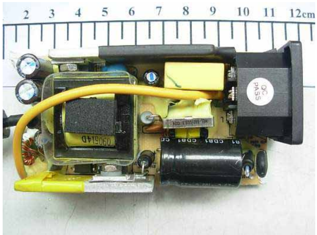
FIGURE 30 LCD MONITOR (M/N: W1930SV) ADAPTER #3 MAIN BOARD (COMPONENT SIDE)
