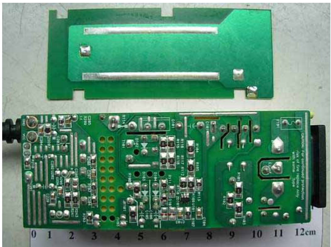
FIGURE 25 LCD MONITOR (M/N: W1930SV) ADAPTER #2 MAIN BOARD (SOLDERED SIDE)
