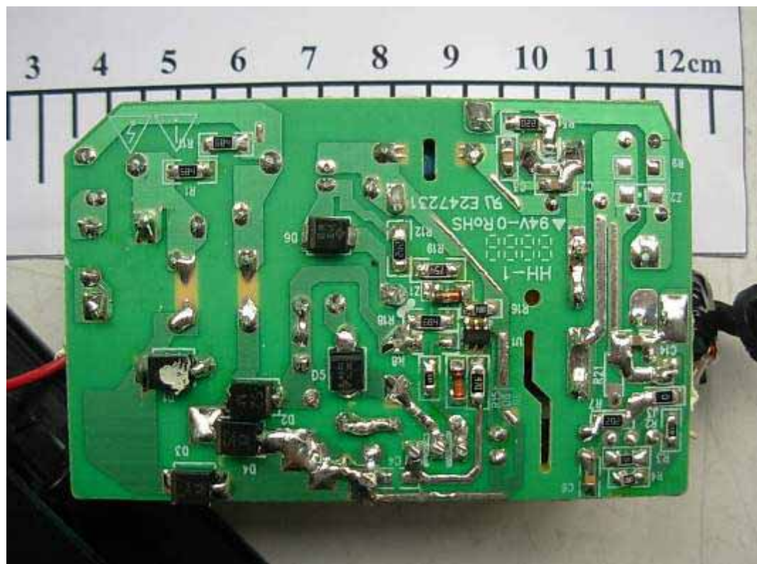
FIGURE 19 LCD MONITOR (M/N: W1930SV) ADAPTER #1 MAIN BOARD (SOLDERED SIDE)
