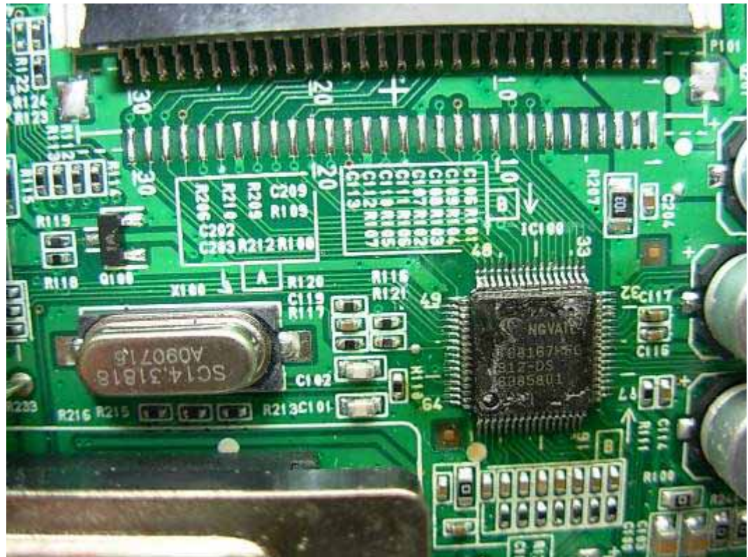
FIGURE 9 LCD MONITOR (M/N: W1930SV) CHIP & CRYSTAL ON MAIN BOARD
