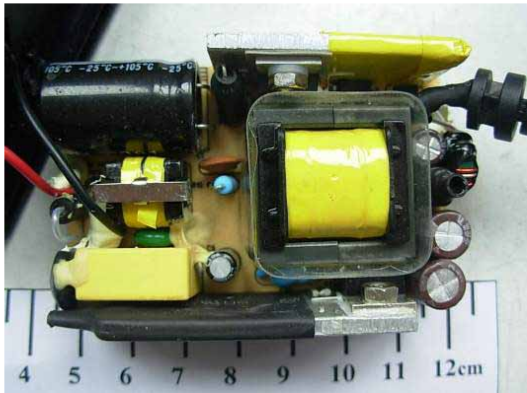
FIGURE 18 LCD MONITOR (M/N: W1930SV) ADAPTER #1 MAIN BOARD (COMPONENT SIDE)
