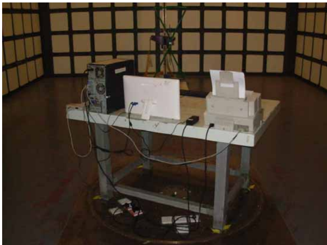
SETUP WITH MAXIMUM DETECTED EMISSION AT VERTICAL POLARIZATION (TEST MODE: D-SUB 1024*768@60Hz, ADAPTER: ADS-24NP-12-1 12024G)
