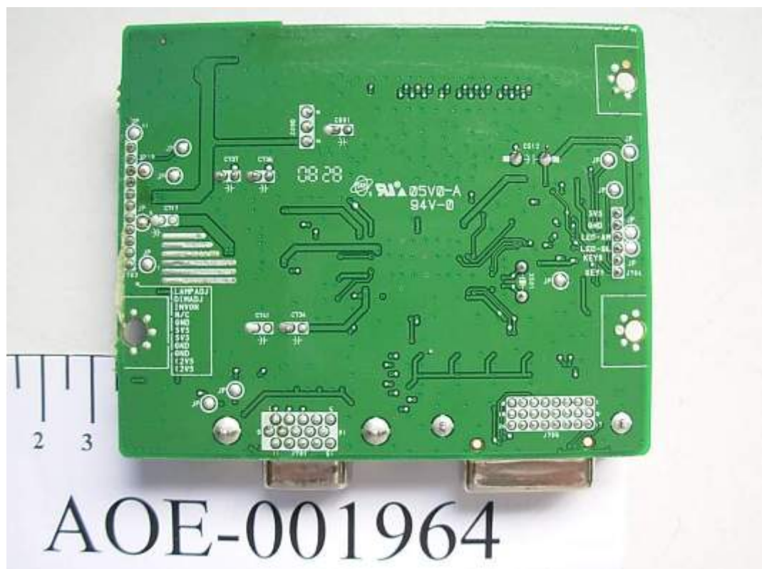
FIGURE 6 LCD MONITOR (M/N: W1942TET) MAIN BOARD (SOLDERED SIDE)
