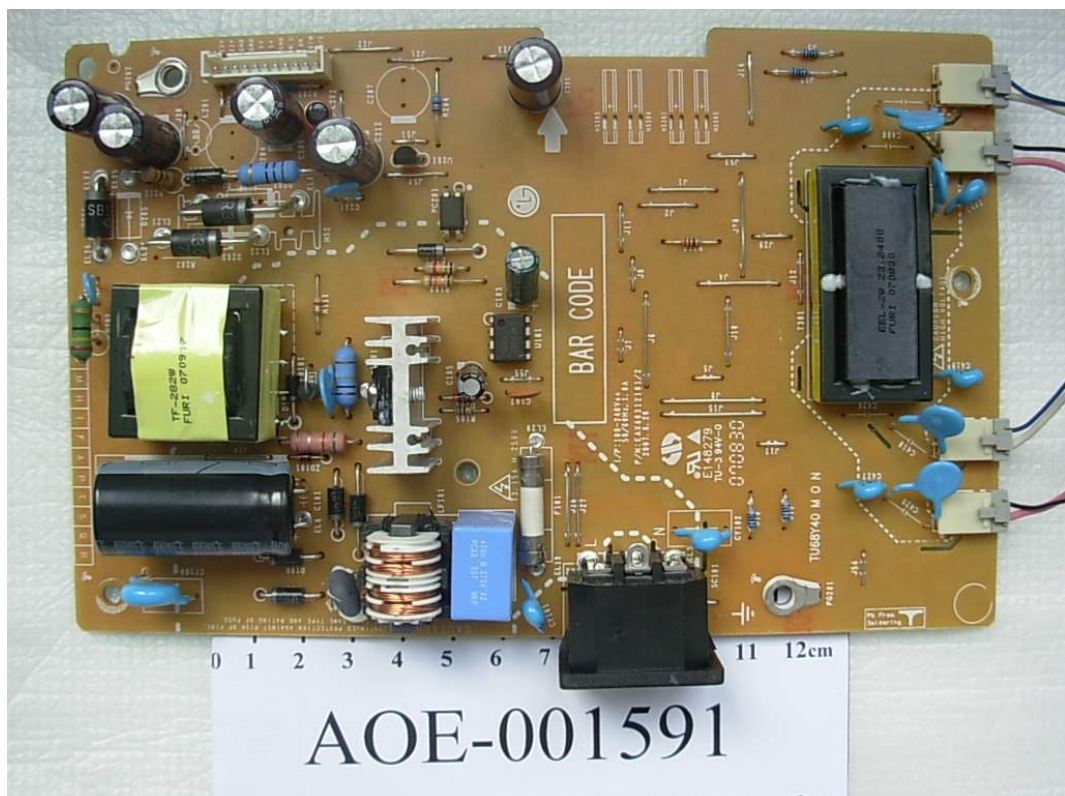
FIGURE 4 LCD MONITOR (M/N: W1942TT) POWER BOARD (COMPONENT SIDE)
