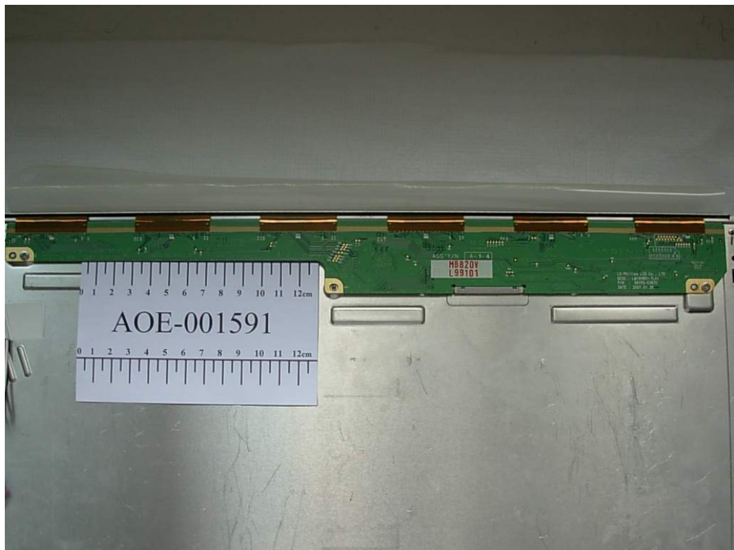
FIGURE 15 LCD MONITOR (M/N: W1942TT) LCD PANEL MAIN BOARD FRONT
