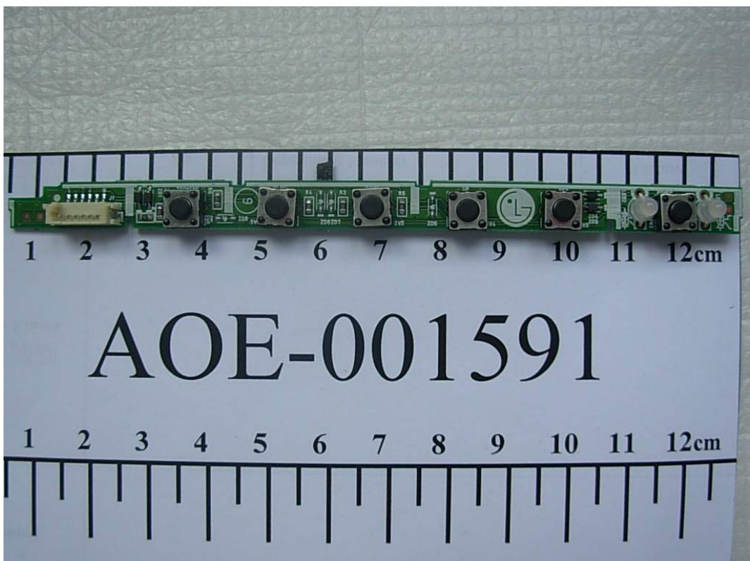
FIGURE 10 LCD MONITOR (M/N: W1942TT) BOTTOM BOARD FRONT
