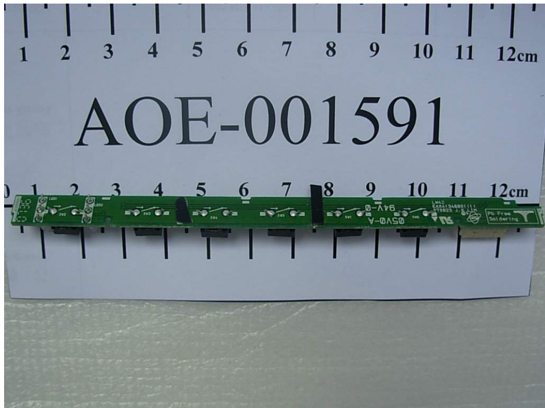
FIGURE 11 LCD MONITOR (M/N: W1942TT) BOTTOM BOARD BACK
