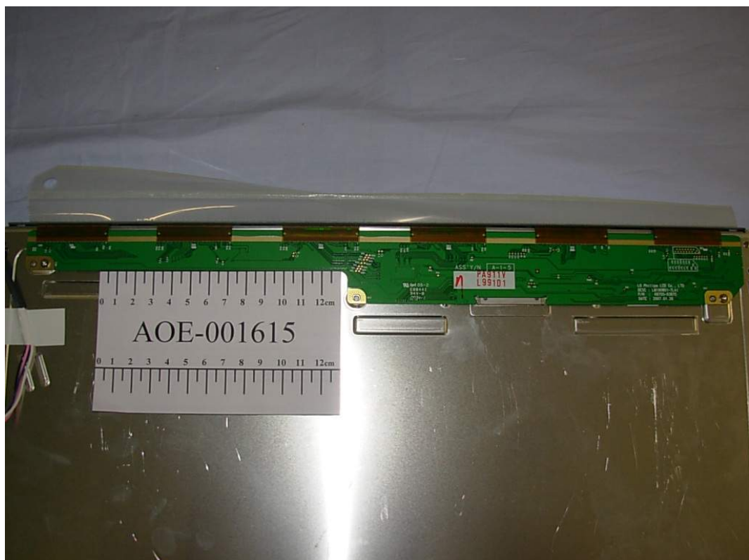
FIGURE 32 LCD MONITOR (M/N: W1942ST) LCD PANEL MAIN BOARD FRONT
