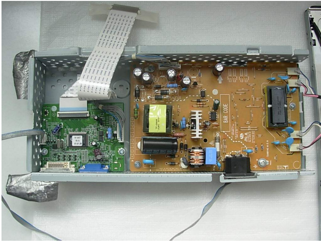
FIGURE 3 LCD MONITOR (M/N: W1942TT) BOARDS INSIDE
