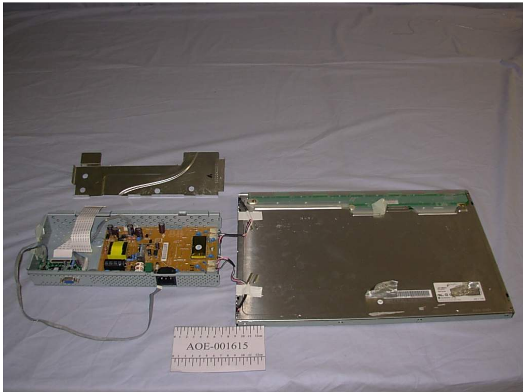
FIGURE 21 LCD MONITOR (M/N: W1942ST) BOARDS REMOVED
