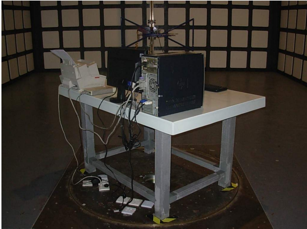
SETUP WITH MAXIMUM DETECTED EMISSION AT HORIZONTAL POLARIZATION (VGA 1440*900@60Hz, Low FREQUENCY)
