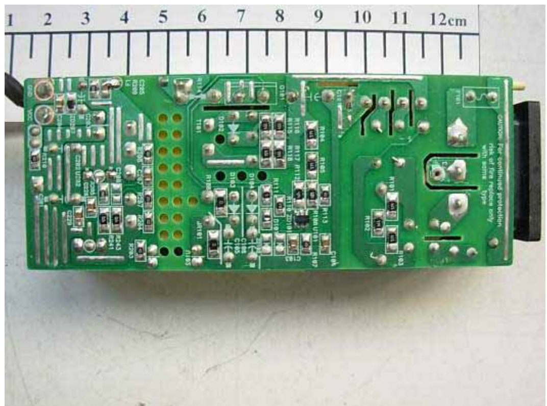
FIGURE 19 LCD MONITOR (M/N: W1943CMV) ADAPTOR MAIN BOARD (SOLDERED SIDE)
