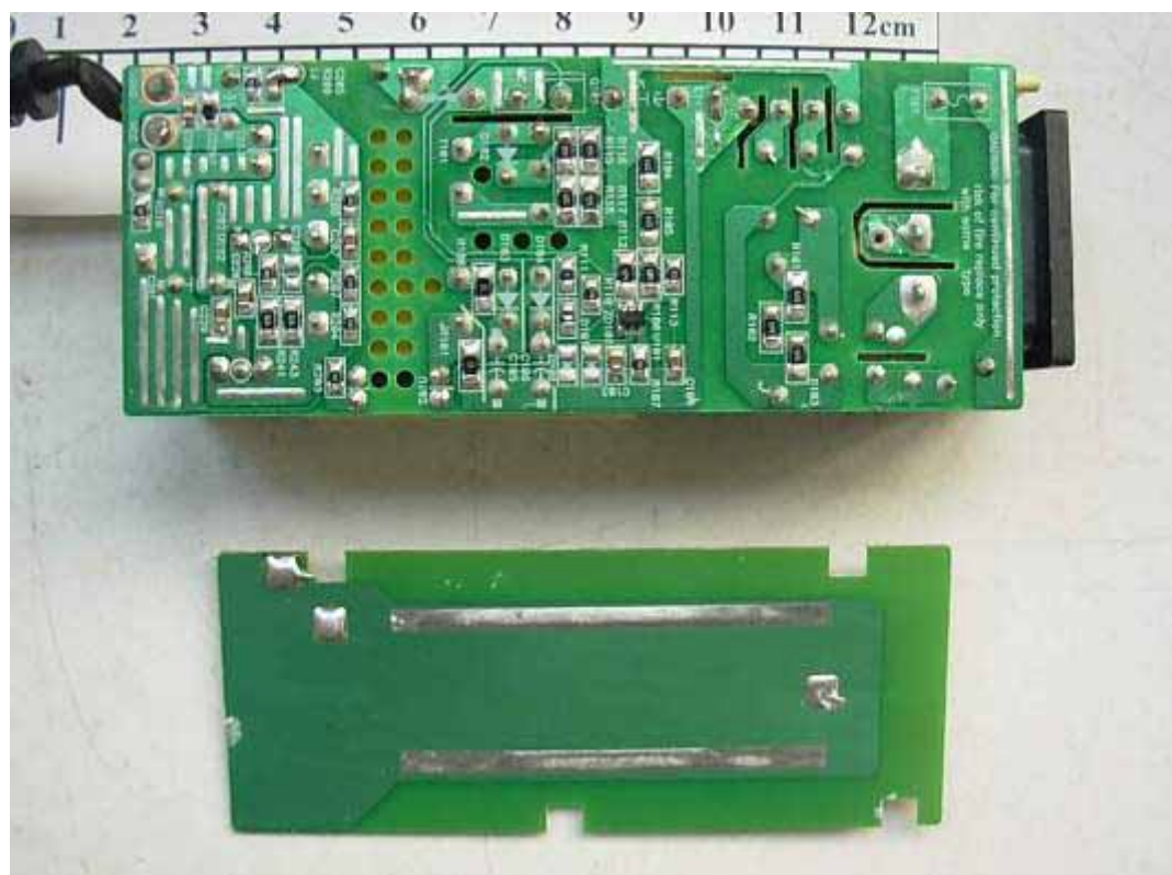
FIGURE 17 LCD MONITOR (M/N: W1943CMV) ADAPTOR GROUNDING BOARD REMOVED
