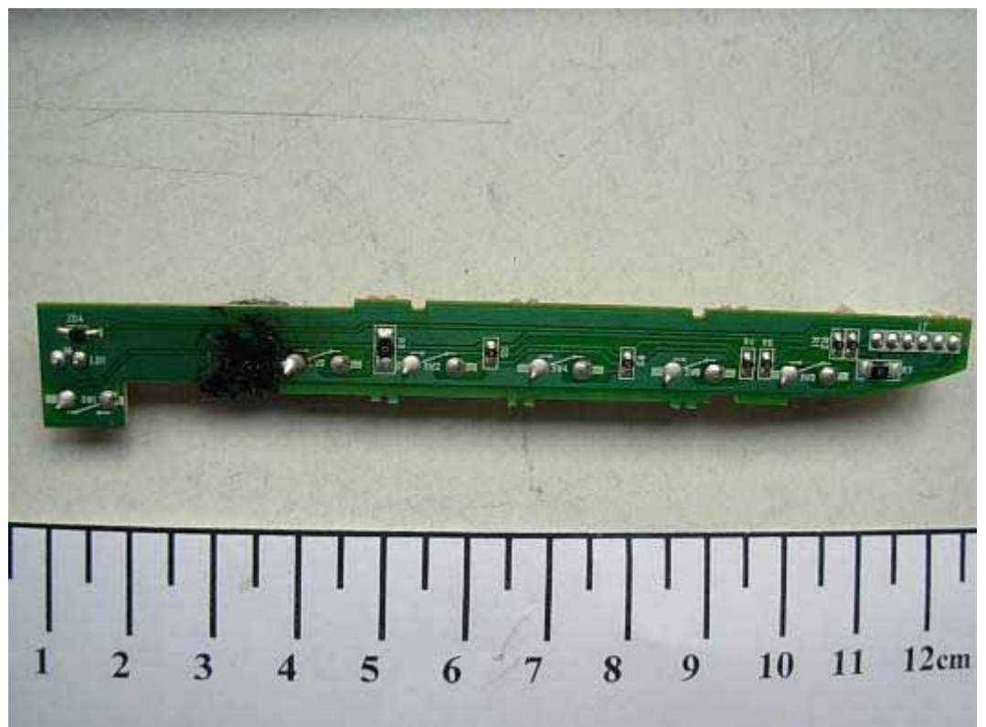
FIGURE 3 LCD MONITOR (M/N: W1943CMV) KEYBOARD (SOLDERED SIDE)
