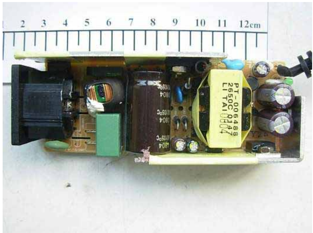
FIGURE 18 LCD MONITOR (M/N: W1943CMV) ADAPTOR MAIN BOARD (COMPONENT SIDE)
