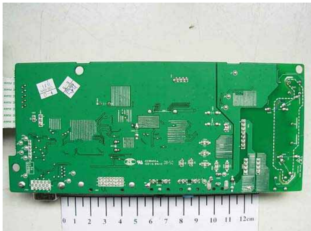
FIGURE 5 LCD MONITOR (M/N: W1943CMV) MAIN BOARD (SOLDERED SIDE)
