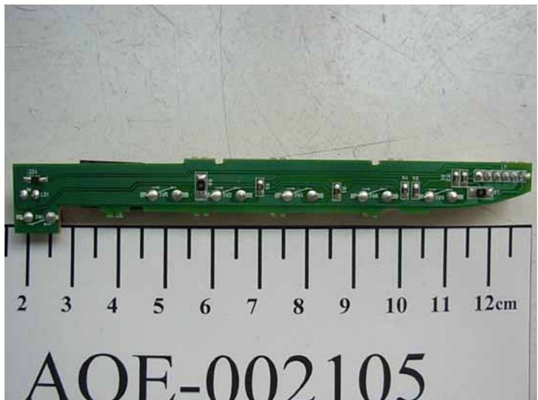
FIGURE 4 LCD MONITOR (M/N: W1943SV) KEY BOARD (SOLDERED SIDE)
