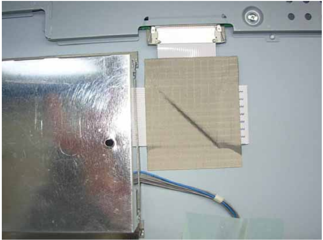
FIGURE 28 LCD MONITOR (M/N: W1943CV) DEBUG #1
