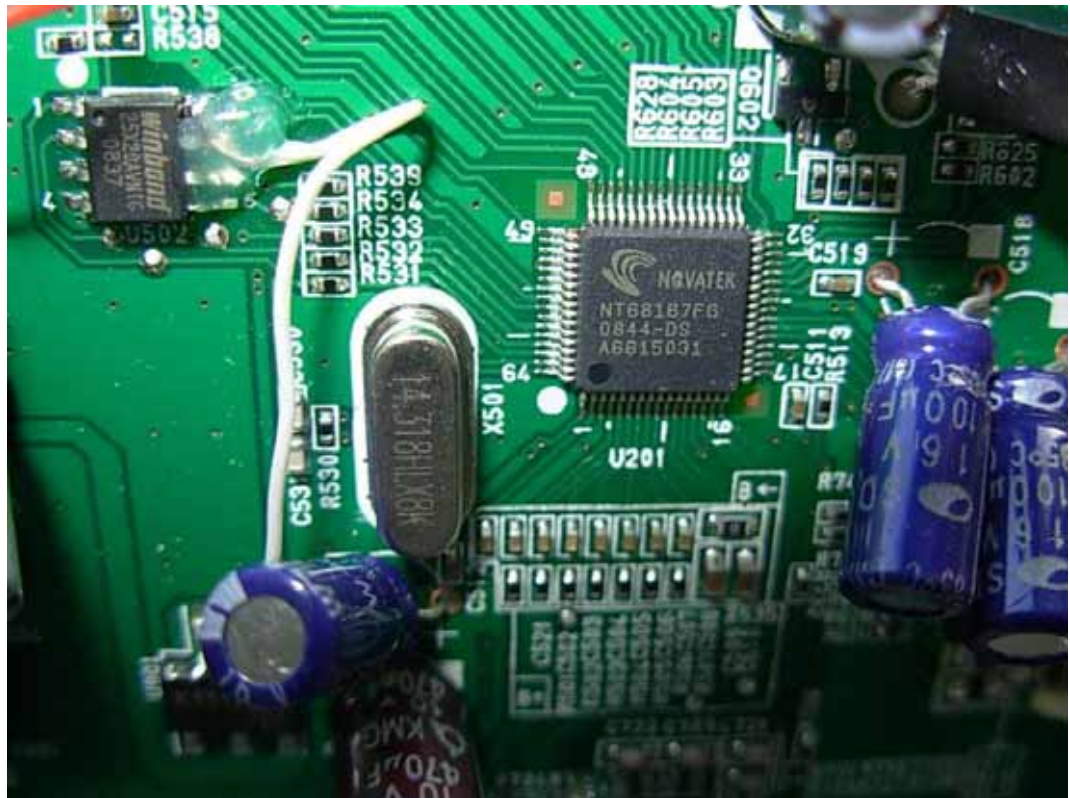
FIGURE 21 LCD MONITOR (M/N: W1943CV) CHIP & CRYSTAL ON MAIN BOARD
