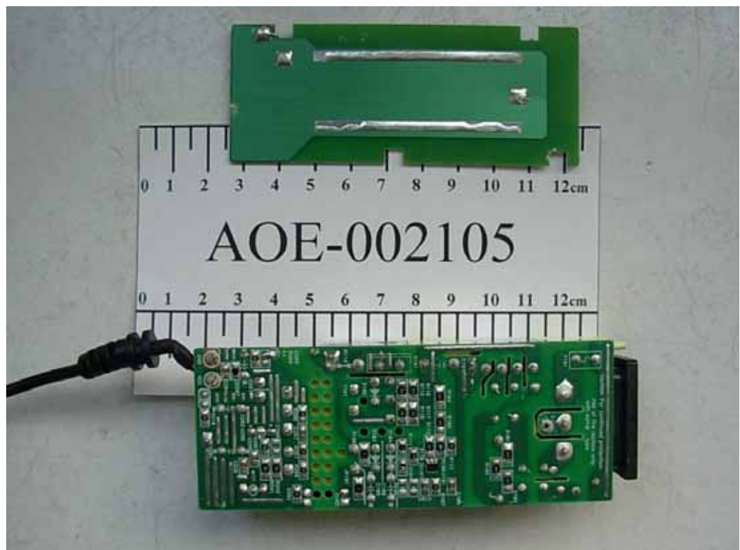
FIGURE 34 LCD MONITOR (M/N: W1943SV, W1943CV) ADAPTOR #1 GROUNDING BOARD REMOVED
