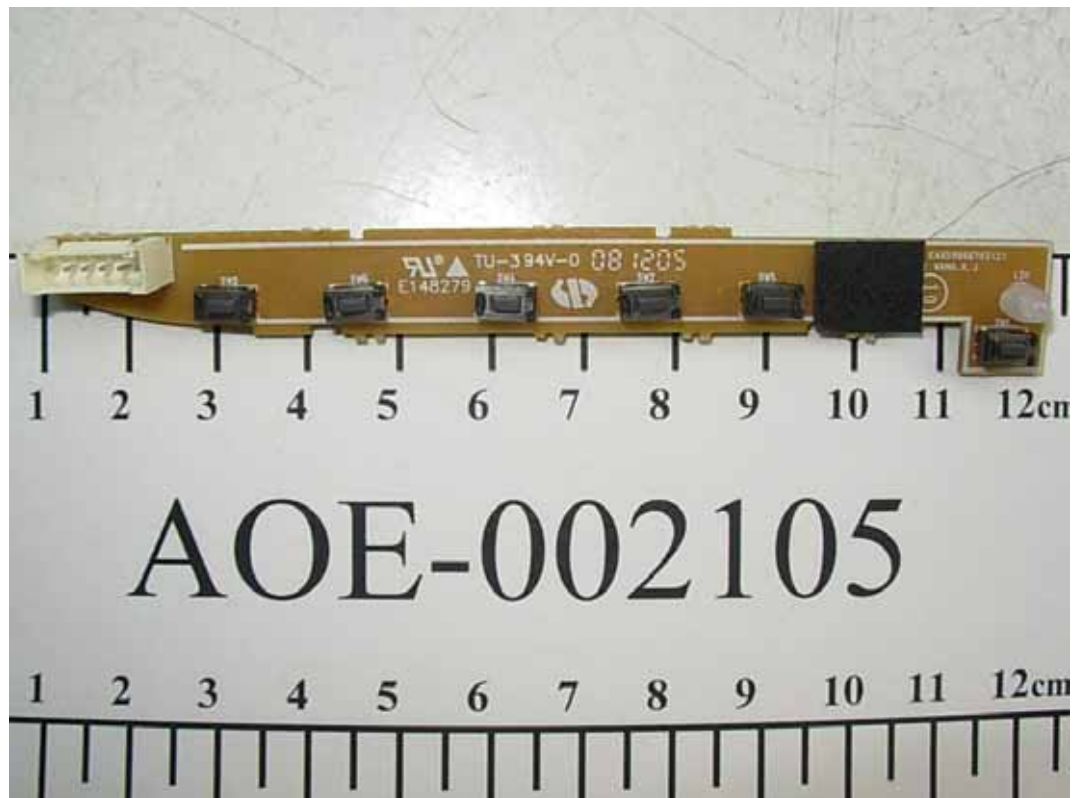
FIGURE 17 LCD MONITOR (M/N: W1943CV) KEYBOARD (COMPONENT SIDE)
