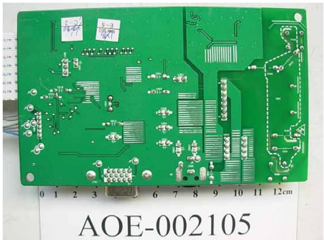
FIGURE 20 LCD MONITOR (M/N: W1943CV) MAIN BOARD (SOLDERED SIDE)
