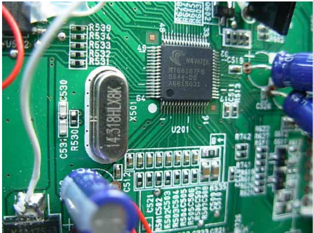
FIGURE 7 LCD MONITOR (M/N: W1943SV) CHIP & CRYSTAL ON MAIN BOARD
