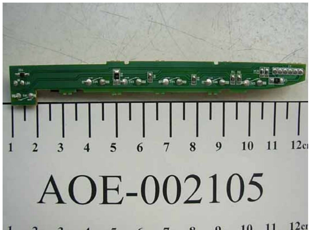
FIGURE 18 LCD MONITOR (M/N: W1943CV) KEYBOARD (SOLDERED SIDE)
