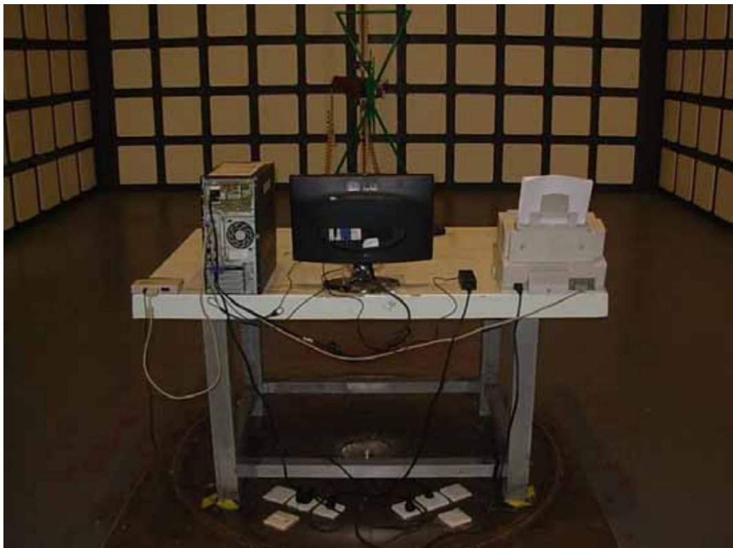
BACK VIEW OF RADIATED EMISSION TEST (ADAPTOR: LCAP07F)
