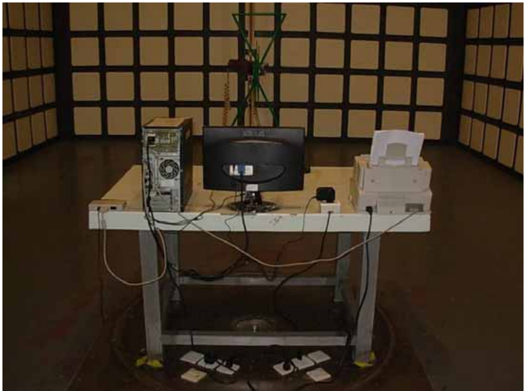
BACK VIEW OF RADIATED EMISSION TEST (ADAPTOR: ADS-24S-12 1224GPCN)
