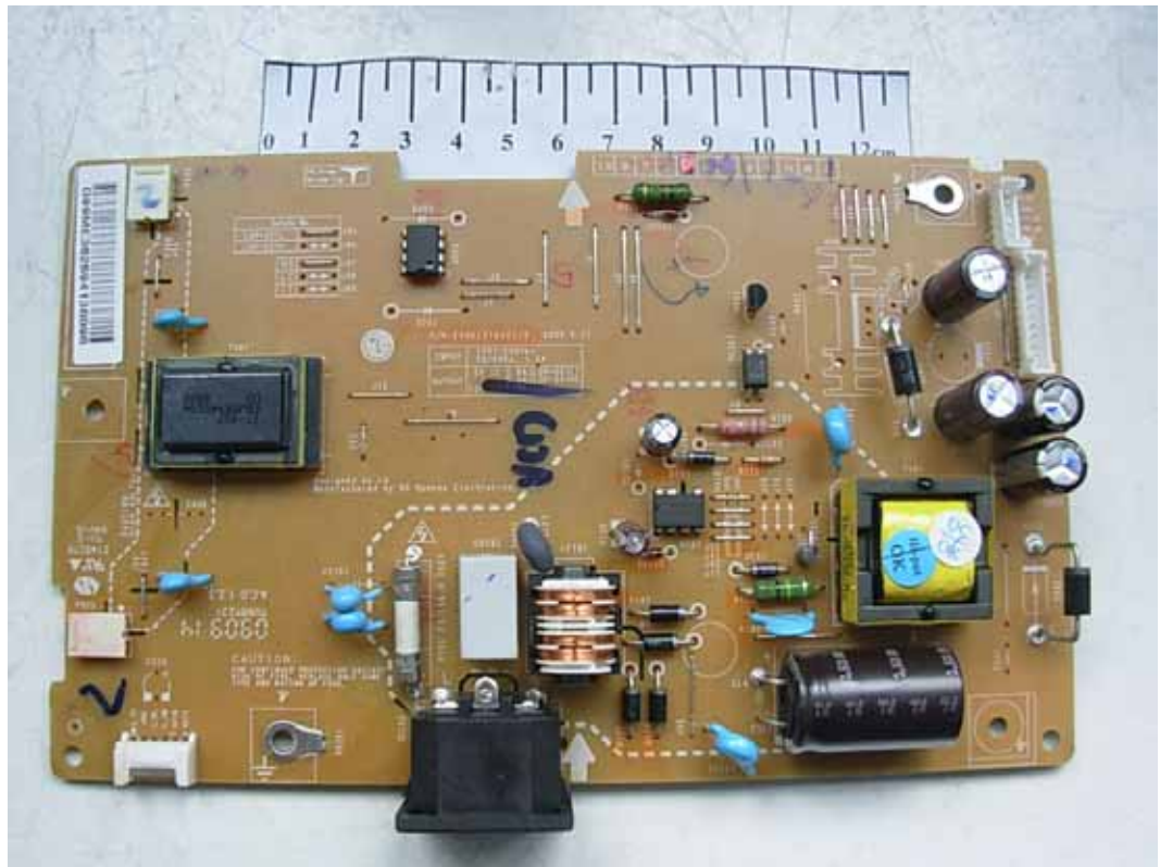
FIGURE 7 LCD MONITOR (M/N: W1946SW) POWER BOARD (COMPONENT SIDE)
