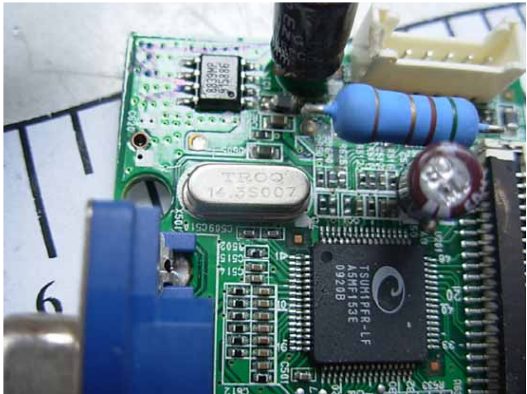
FIGURE 4 LCD MONITOR (M/N: W1946SW) CHIP & CRYSTAL ON MAIN BOARD
