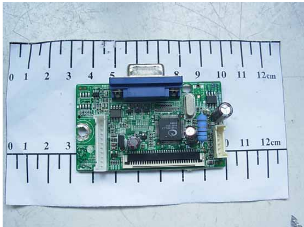
FIGURE 2 LCD MONITOR (M/N: W1946SW) MAIN BOARD (COMPONENT SIDE)
