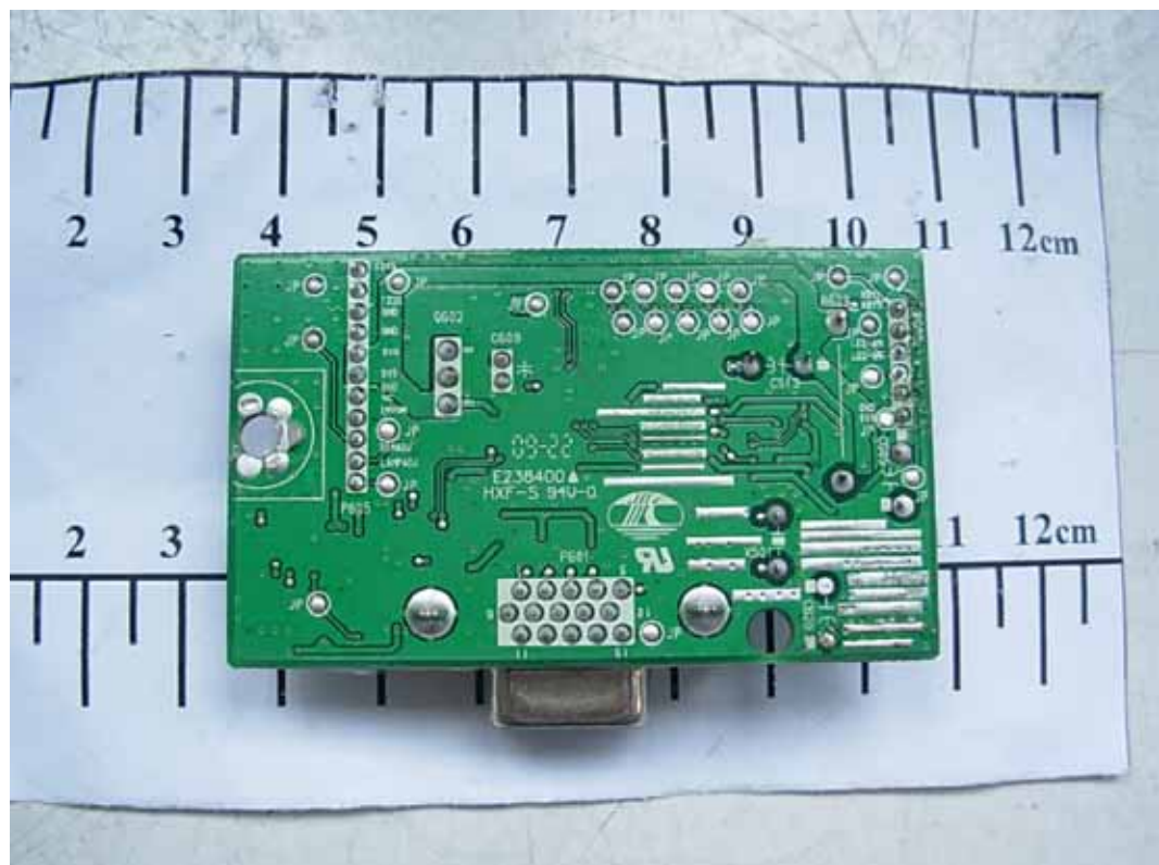
FIGURE 3 LCD MONITOR (M/N: W1946SW) MAIN BOARD (SOLDERED SIDE)
