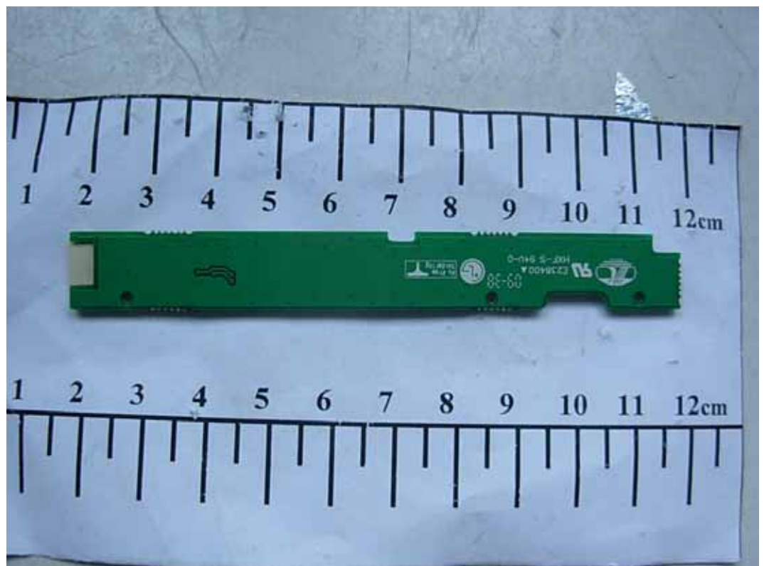
FIGURE 6 LCD MONITOR (M/N: W1946SW) KEY BOARD (SOLDERED SIDE)
