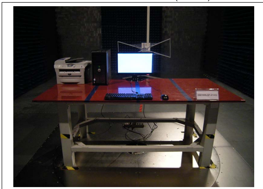
Front View of Radiated Emission Test (Under 1G)
