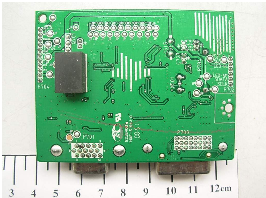
FIGURE 10 LCD MONITOR (M/N: W2061TQV) MAIN BOARD (SOLDERED SIDE)
