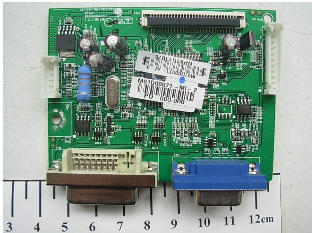
FIGURE 9 LCD MONITOR (M/N: W2061TQV) MAIN BOARD (COMPONENT SIDE)
