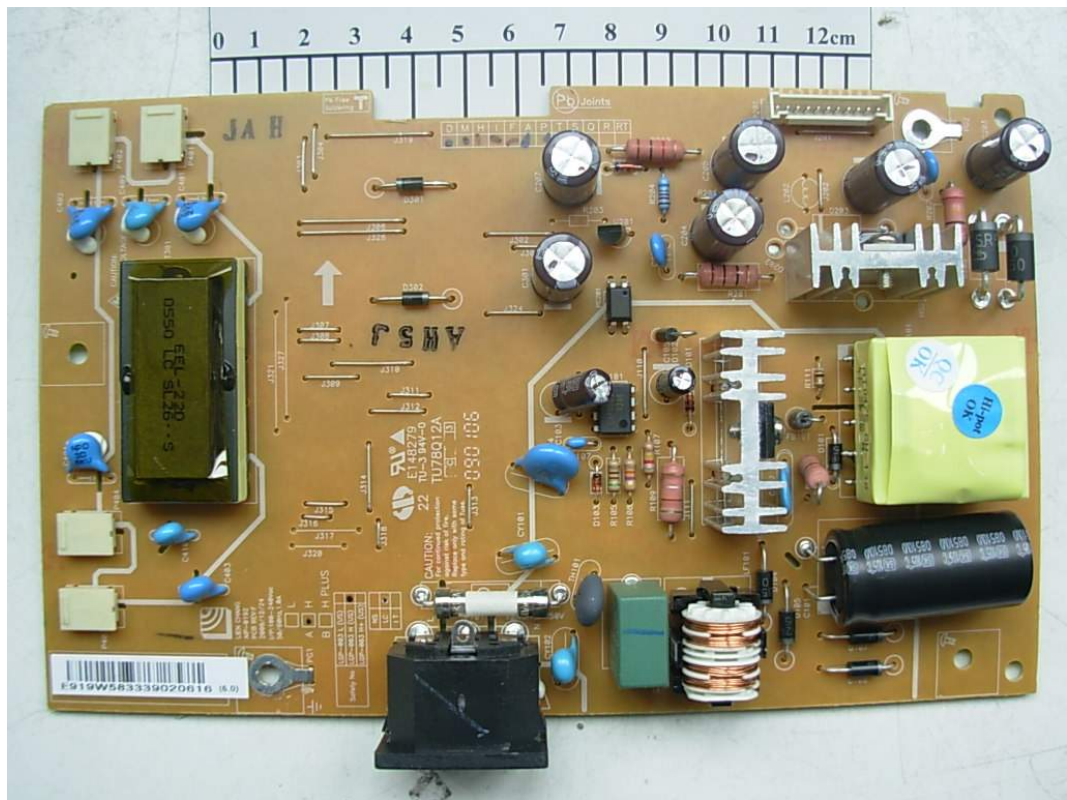
FIGURE 7 LCD MONITOR (M/N: W2061TQV) POWER BOARD (COMPONENT SIDE)
