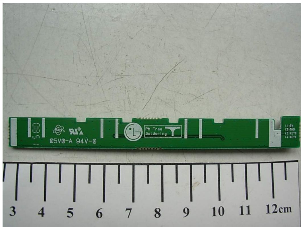
FIGURE 4 LCD MONITOR (M/N: W2061TQV) KEYBOARD (SOLDERED SIDE)
