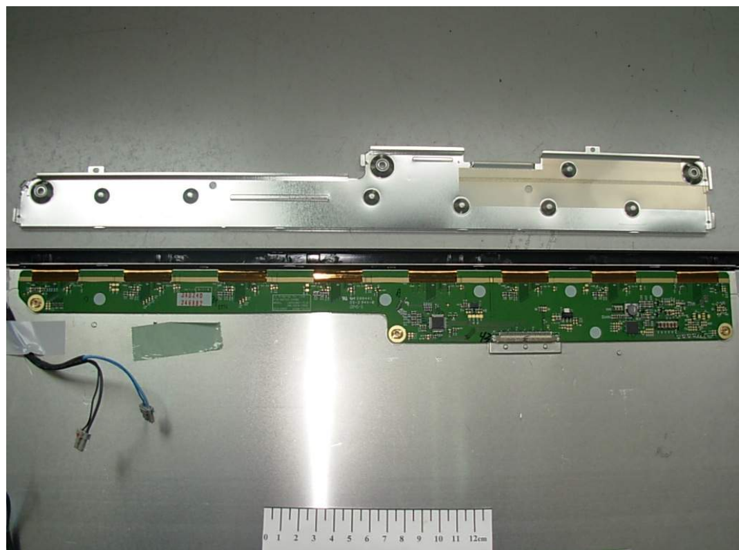
FIGURE 13 LCD MONITOR (M/N: W2061TQV) LCD PANEL MAIN BOARD COVER REMOVED
