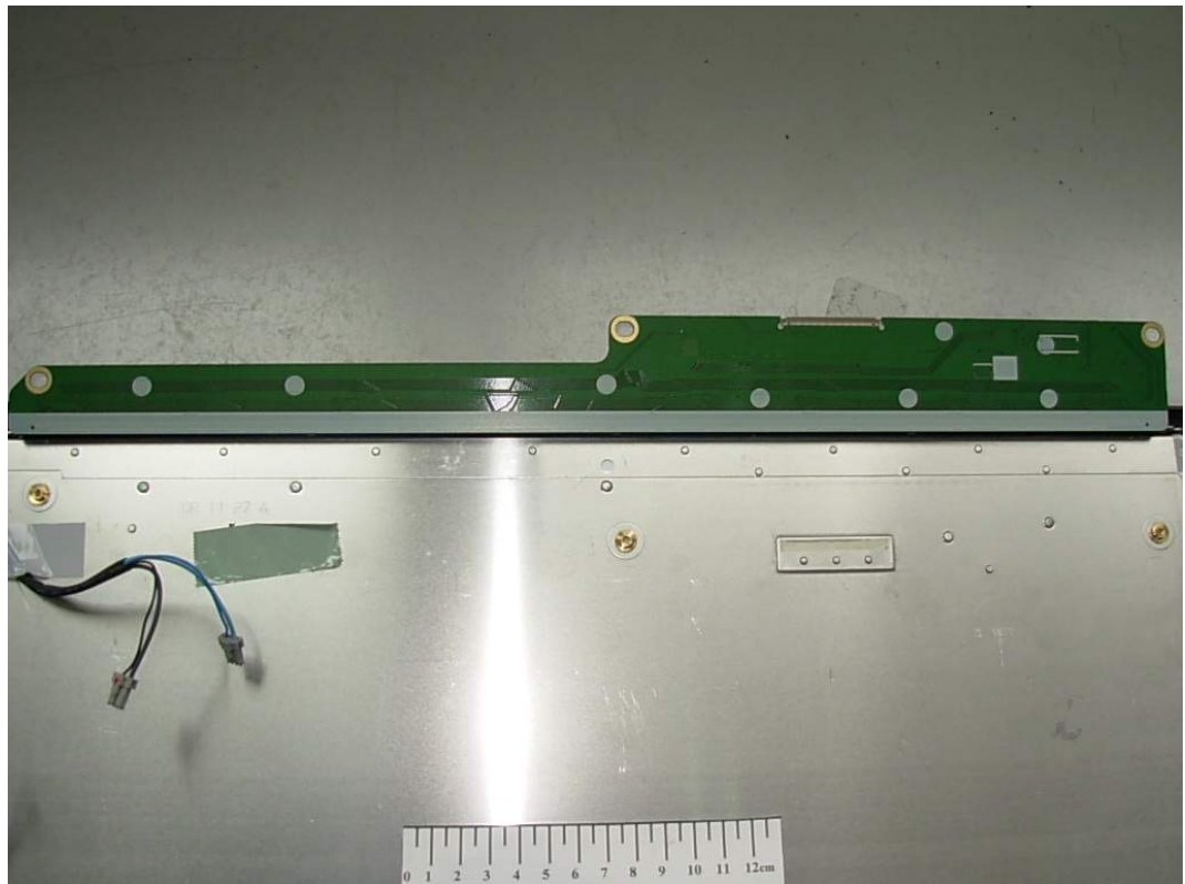
FIGURE 14 LCD MONITOR (M/N: W2061TQV) LCD PANEL MAIN BOARD (SOLDERED SIDE)
