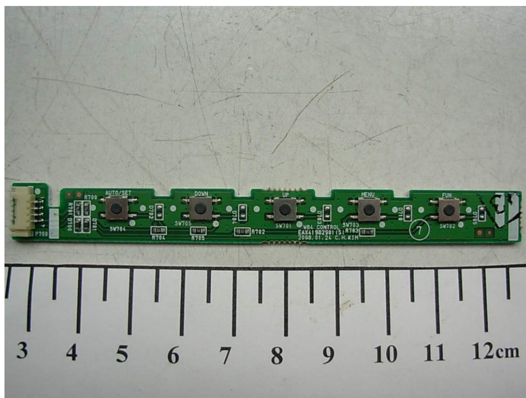
FIGURE 3 LCD MONITOR (M/N: W2061TQV) KEYBOARD (COMPONENT SIDE)
