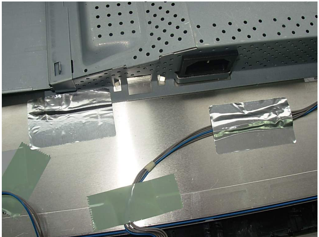
FIGURE 17 LCD MONITOR (M/N: W2061TQV) DEBUG #1
