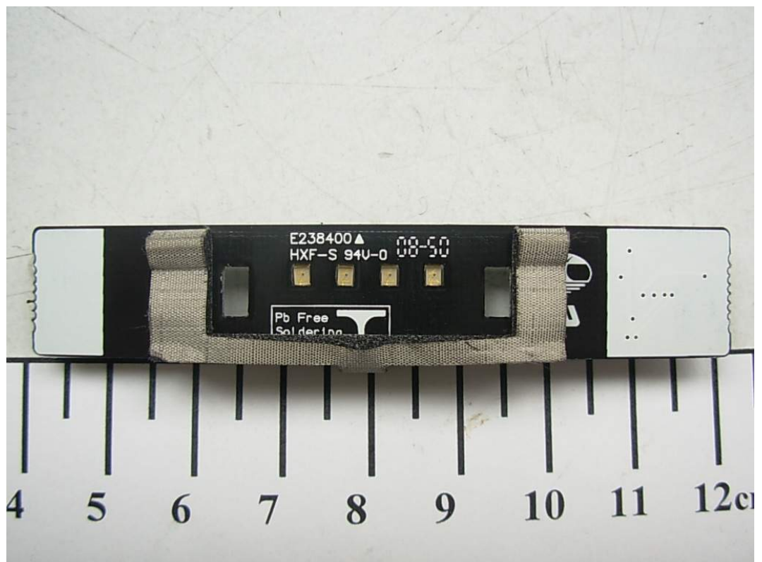
FIGURE 6 LCD MONITOR (M/N: W2061TQV) LED BOARD (SOLDERED SIDE)
