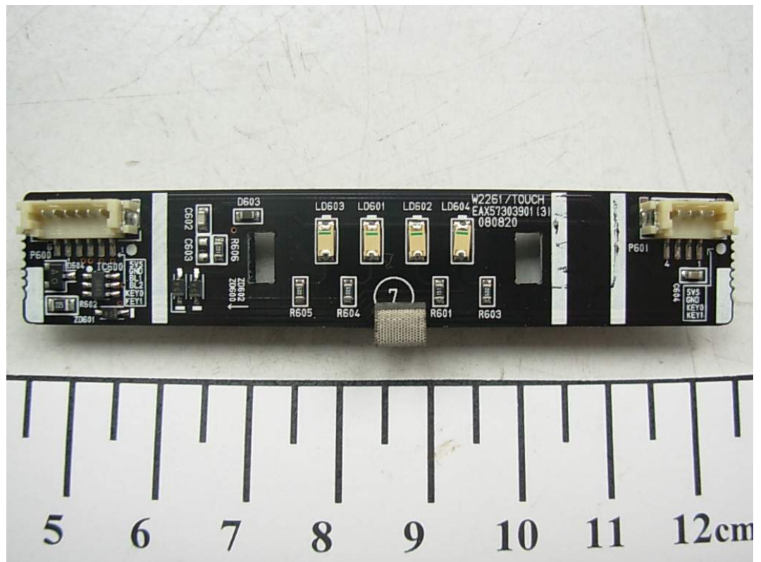
FIGURE 5 LCD MONITOR (M/N: W2061TQV) LED BOARD (COMPONENT SIDE)
