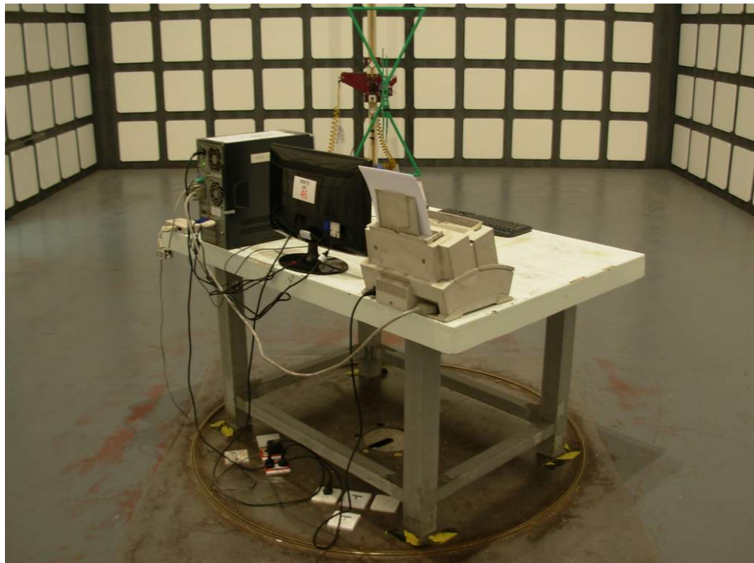
SETUP WITH MAXIMUM DETECTED EMISSION AT VERTICAL POLARIZATION (DVI 1600*900@60Hz)
