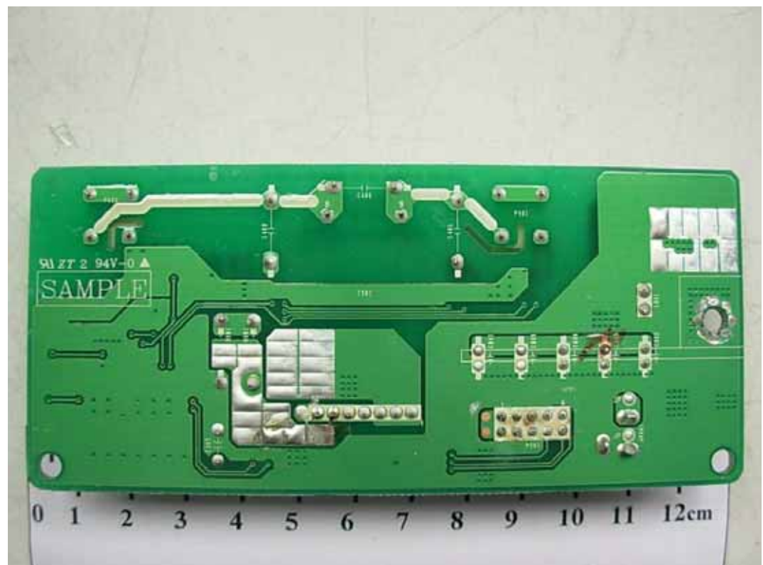
FIGURE 6 LCD MONITOR (M/N: W2230SV) POWER BOARD (SOLDERED SIDE)
