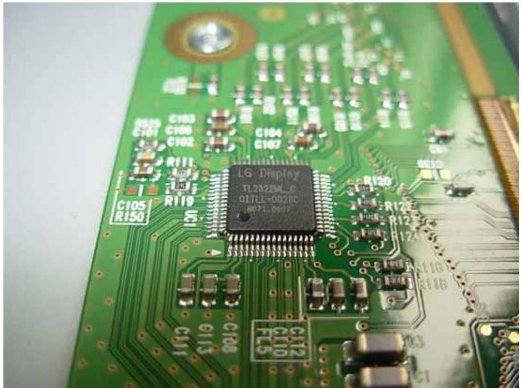
FIGURE 13 LCD MONITOR (M/N: W2230SV) CHIP ON LCD PANEL MAIN BOARD
