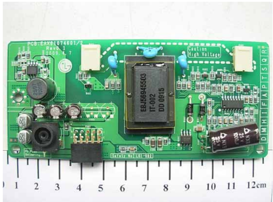
FIGURE 5 LCD MONITOR (M/N: W2230SV) POWER BOARD (COMPONENT SIDE)
