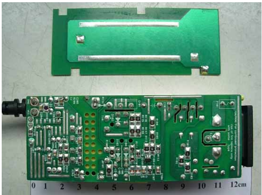
FIGURE 20 LCD MONITOR (M/N: W2230SV) ADAPTER MAIN BOARD (SOLDERED SIDE)
