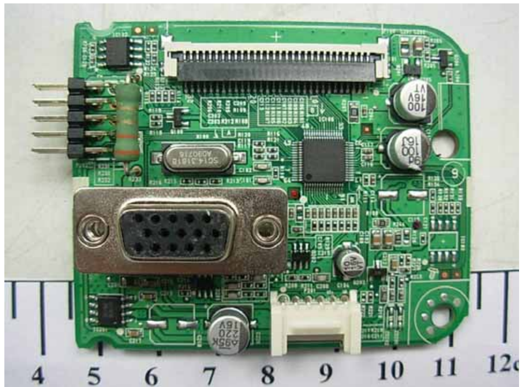
FIGURE 7 LCD MONITOR (M/N: W2230SV) MAIN BOARD (COMPONENT SIDE)
