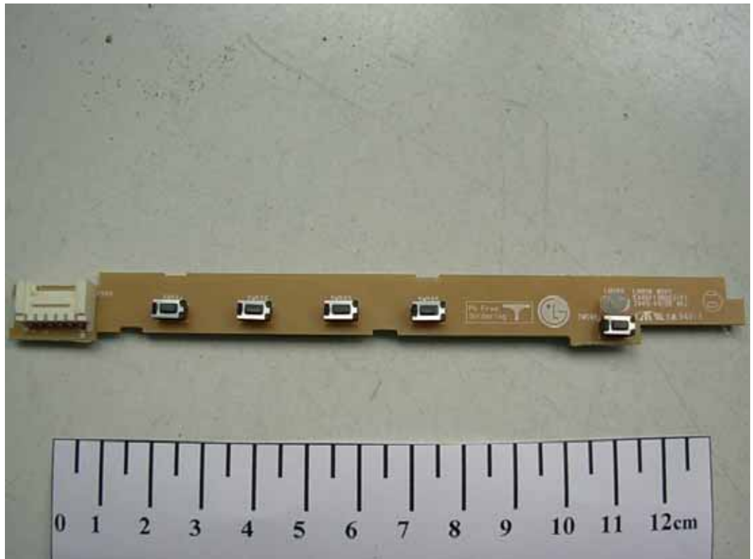
FIGURE 3 LCD MONITOR (M/N: W2230SV) KEYBOARD (COMPONENT SIDE)
