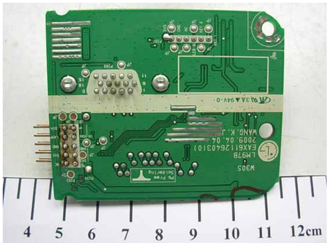
FIGURE 8 LCD MONITOR (M/N: W2230SV) MAIN BOARD (SOLDERED SIDE)
