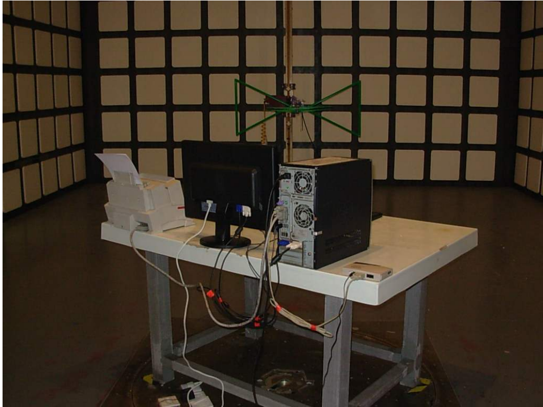
SETUP WITH MAXIMUM DETECTED EMISSION AT HORIZONTAL POLARIZATION (VGA 1024*768@60Hz, M/N: W2241TT)
