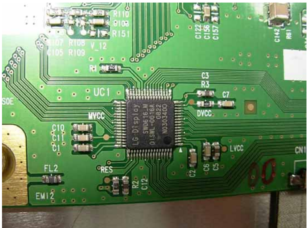
FIGURE 14 LCD MONITOR (M/N: W2242TET) LCD PANEL MAIN BOARD CHIP
