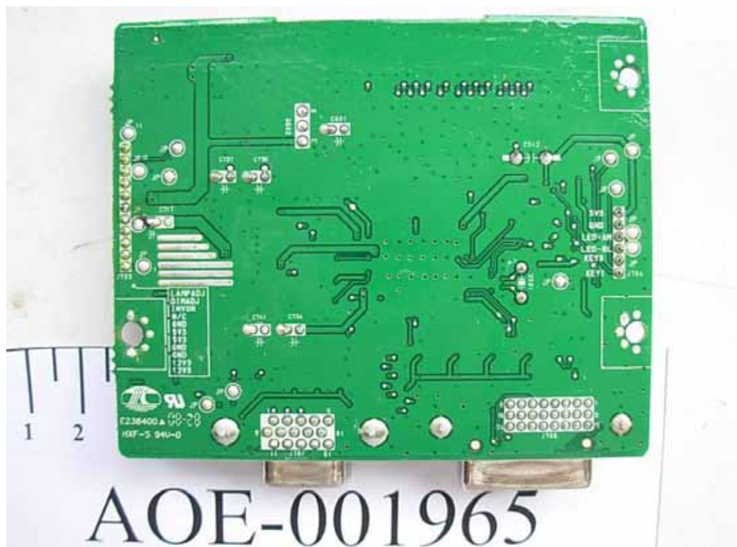
FIGURE 6 LCD MONITOR (M/N: W2242TET) MAIN BOARD (SOLDERED SIDE)
