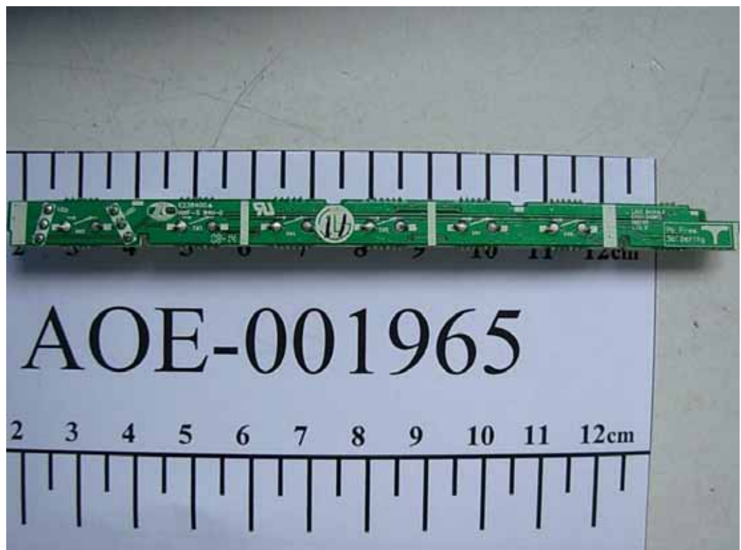
FIGURE 3 LCD MONITOR (M/N: W2242TET) KEY BOARD (SOLDERED SIDE)
