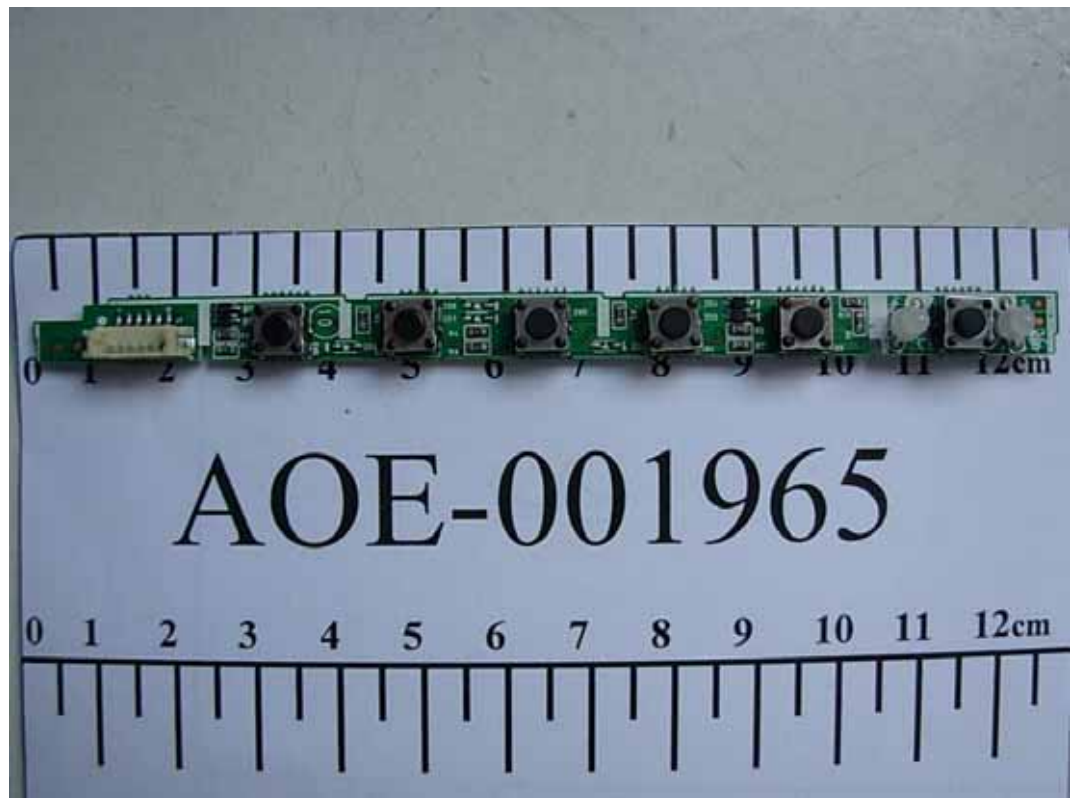
FIGURE 2 LCD MONITOR (M/N: W2242TET) KEY BOARD (COMPONENT SIDE)
