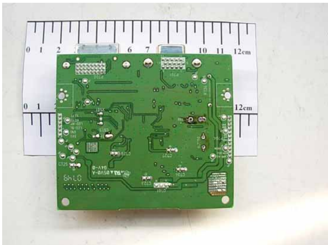
FIGURE 8 LCD MONITOR (M/N: W2242TQT) MAIN BOARD (SOLDERED SIDE)
