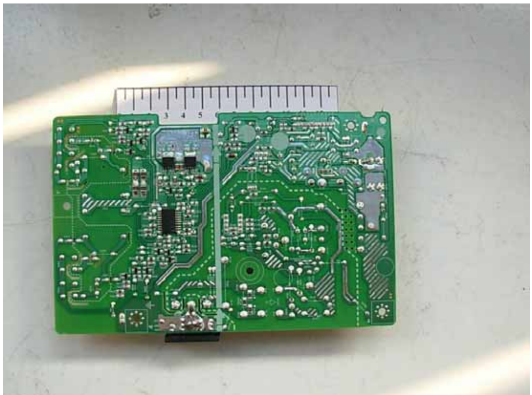
FIGURE 6 LCD MONITOR (M/N: W2242TQT) POWER BOARD (SOLDERED SIDE)
