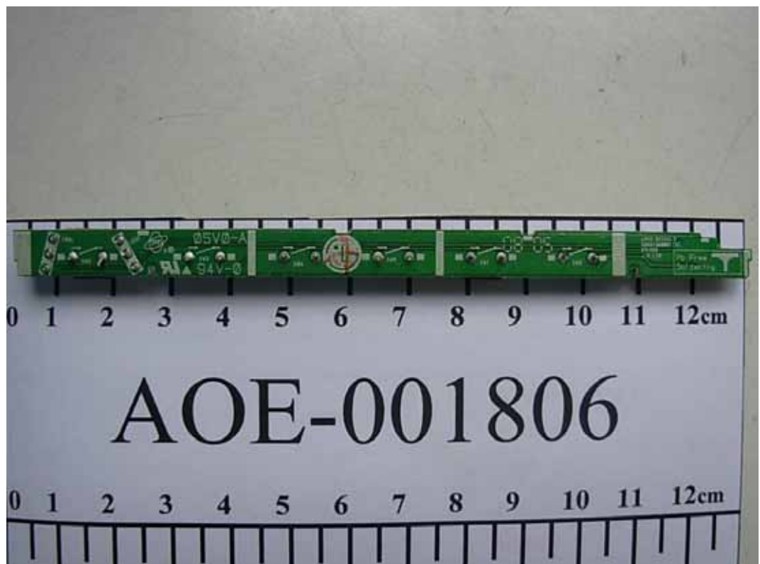
FIGURE 3 LCD MONITOR (M/N: W2242SMT) BUTTON BOARD (SOLDERED SIDE)
