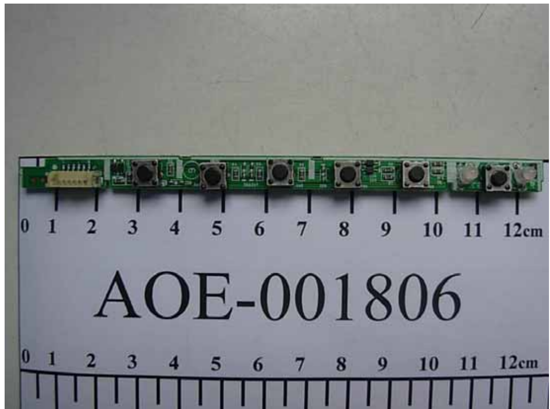
FIGURE 2 LCD MONITOR (M/N: W2242SMT) BUTTON BOARD (COMPONENT SIDE)
