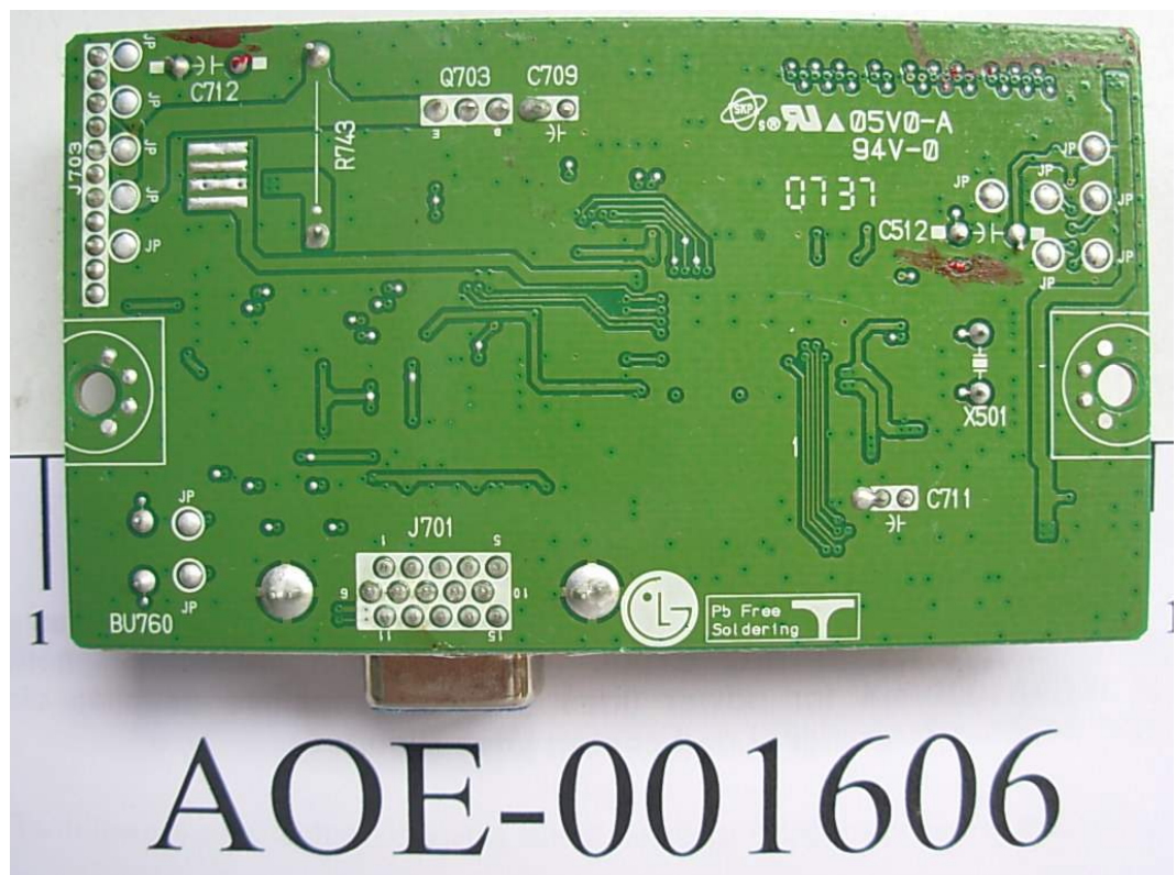
FIGURE 31 LCD MONITOR (M/N: W2252SQT) MAIN BOARD (SOLDERED SIDE)
