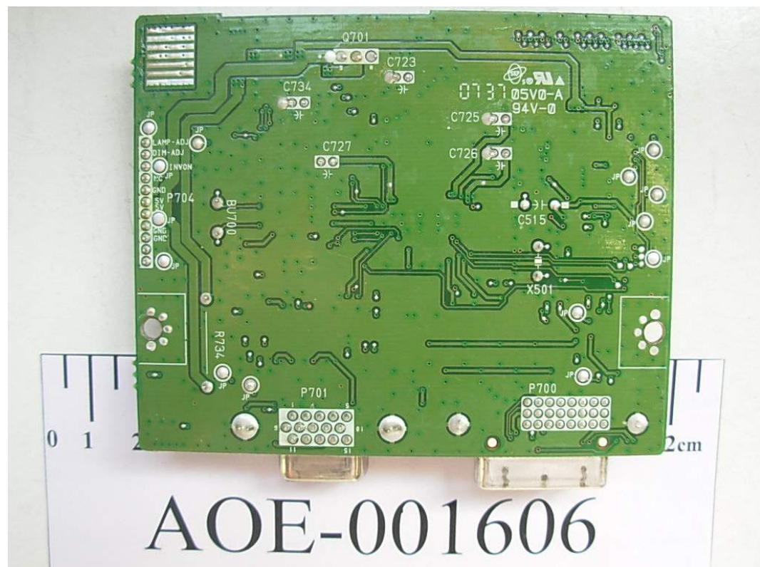
FIGURE 11 LCD MONITOR (M/N: W2252TQT) MAIN BOARD (SOLDERED SIDE)
