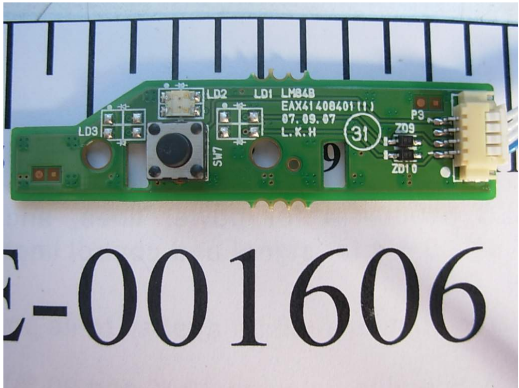
FIGURE 5 LCD MONITOR (M/N: W2252TQT) LED BOARD FRONT
