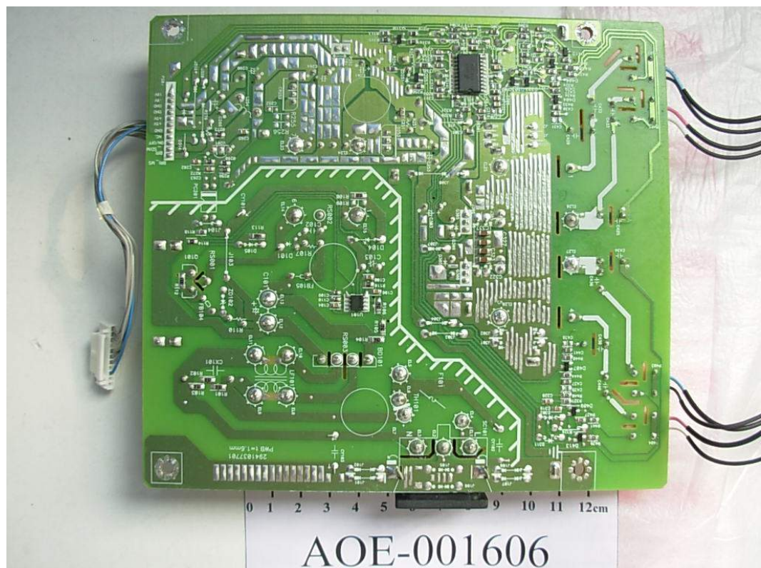
FIGURE 29 LCD MONITOR (M/N: W2252SQT) POWER BOARD (SOLDERED SIDE)
