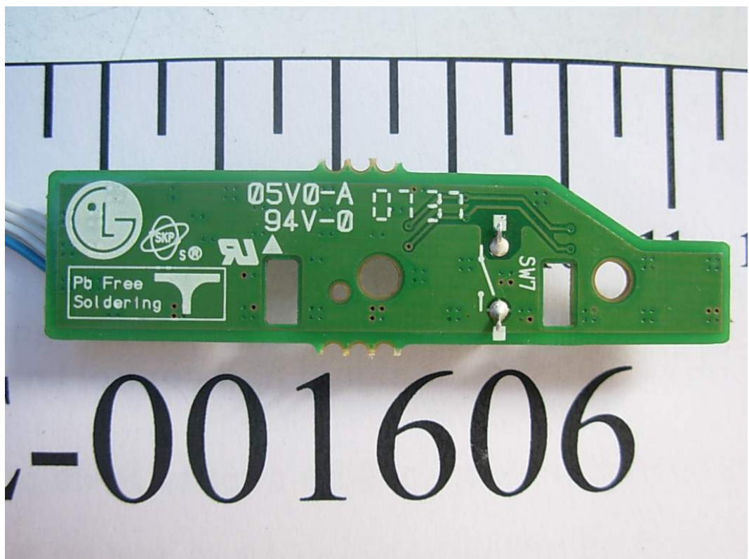
FIGURE 6 LCD MONITOR (M/N: W2252TQT) LED BOARD BACK
