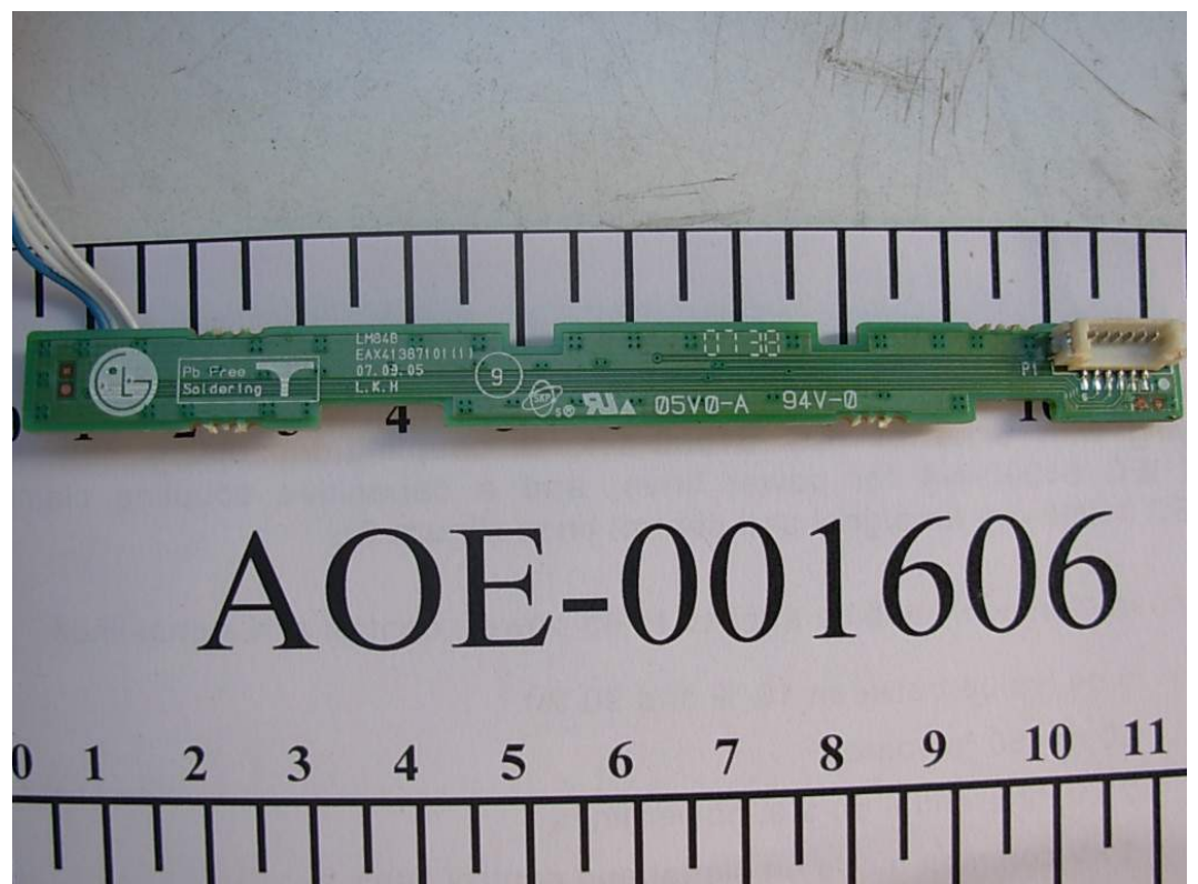
FIGURE 4 LCD MONITOR (M/N: W2252TQT) BUTTON BOARD BACK
