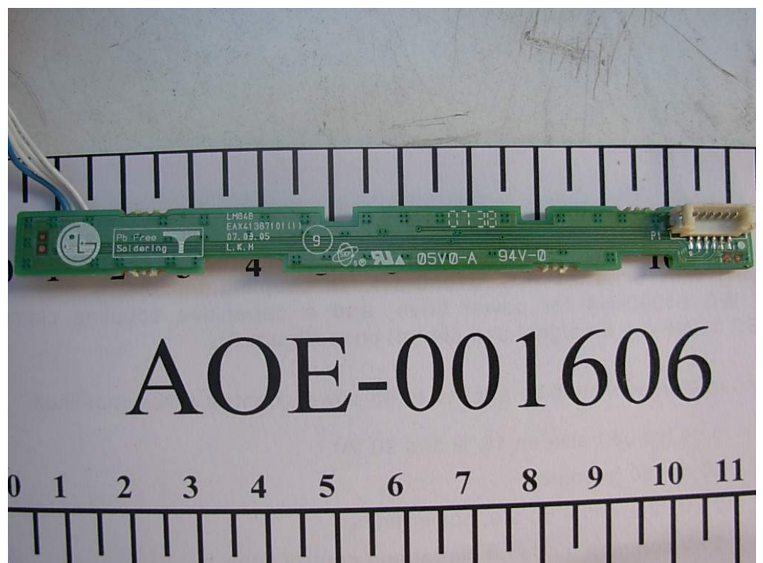
FIGURE 25 LCD MONITOR (M/N: W2252SQT) BUTTON BOARD BACK
