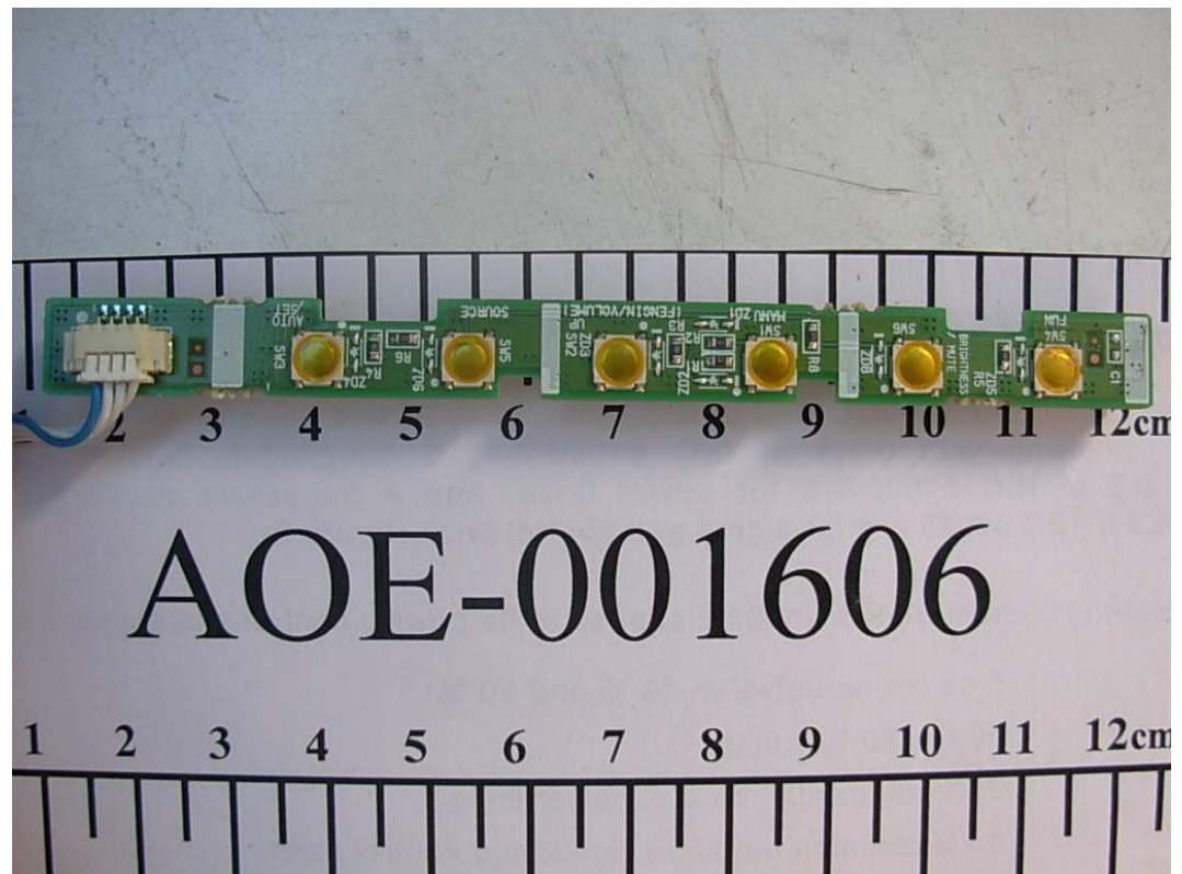
FIGURE 3 LCD MONITOR (M/N: W2252TQT) BUTTON BOARD FRONT
