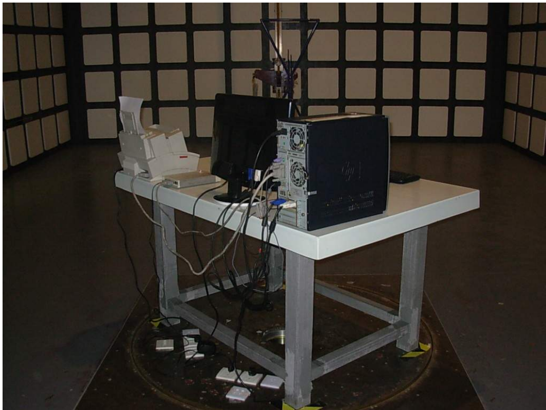
SETUP WITH MAXIMUM DETECTED EMISSION AT VERTICAL POLARIZATION (VGA 1680*1050@60Hz, Low FREQUENCY) (M/N: W2252TQT)
