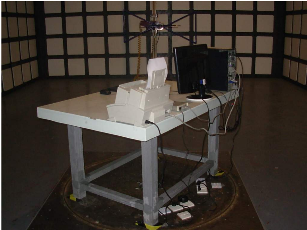
SETUP WITH MAXIMUM DETECTED EMISSION AT HORIZONTAL POLARIZATION (VGA 1680*1050@60Hz, Low FREQUENCY) (M/N: W2252TQT)
