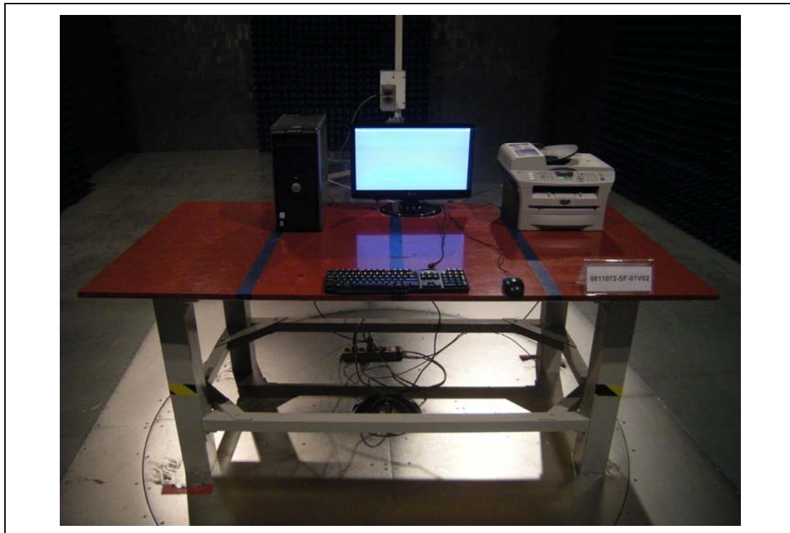
Front View of Radiated Emission Test (Above 1G)
