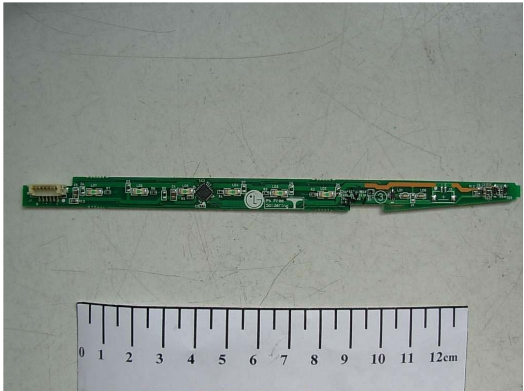
FIGURE 4 LCD MONITOR (M/N: W2254VQV) KEYBOARD (COMPONENT SIDE)
