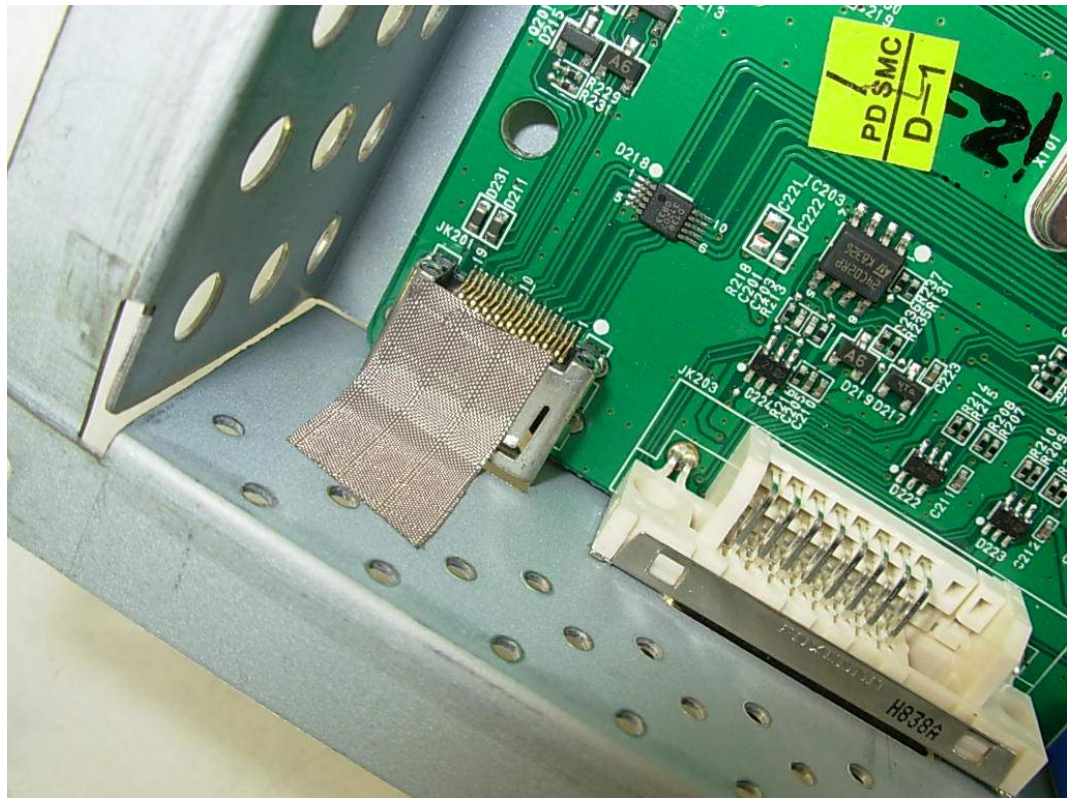
FIGURE 18 LCD MONITOR (M/N: W2254VQV) DEBUG #3
