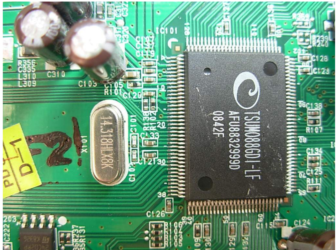
FIGURE 8 LCD MONITOR (M/N: W2254VQV) CHIP & CRYSTAL ON MAIN BOARD
