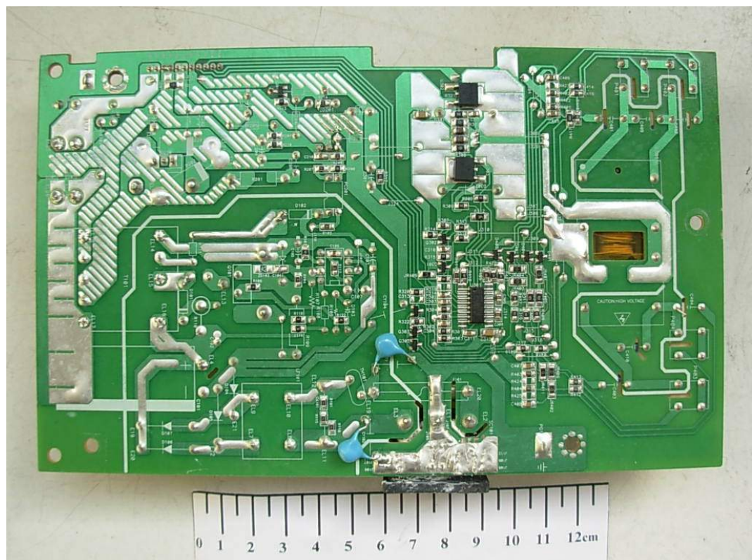
FIGURE 10 LCD MONITOR (M/N: W2254VQV) POWER BOARD (SOLDERED SIDE)
