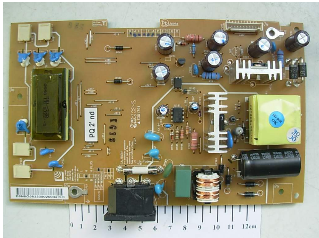
FIGURE 9 LCD MONITOR (M/N: W2254VQV) POWER BOARD (COMPONENT SIDE)
