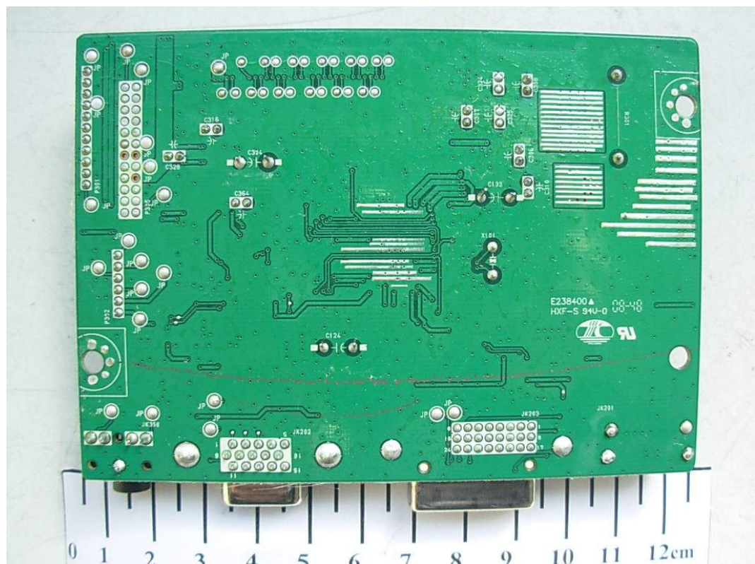
FIGURE 7 LCD MONITOR (M/N: W2254VQV) MAIN BOARD (SOLDERED SIDE)
