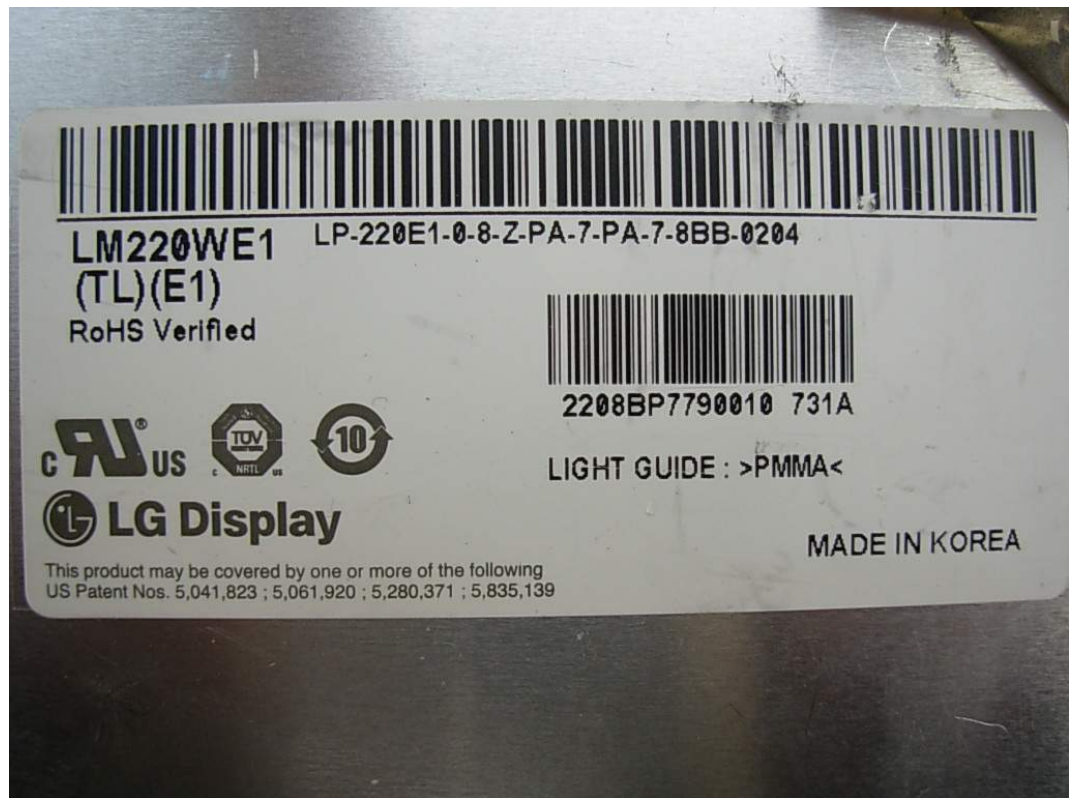
FIGURE 11 LCD MONITOR (M/N: W2254VQV) LCD PANEL LABEL
