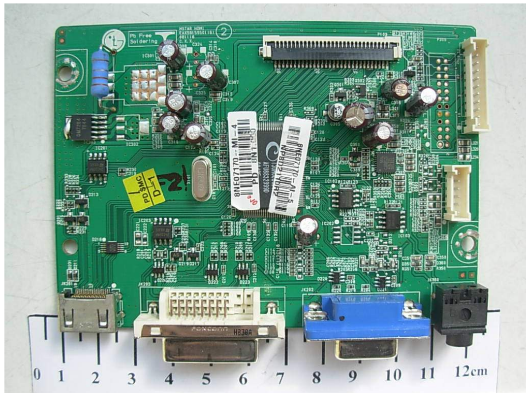
FIGURE 6 LCD MONITOR (M/N: W2254VQV) MAIN BOARD (COMPONENT SIDE)
