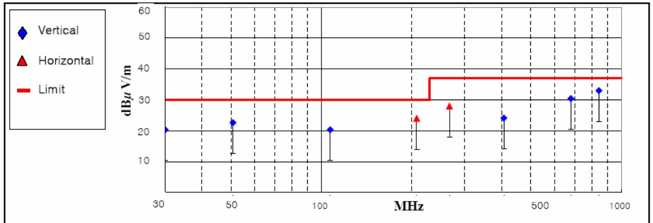
&lt; Fig 8. Radiated emission result (30 MHz ~ 1 000 MHz)&gt;
