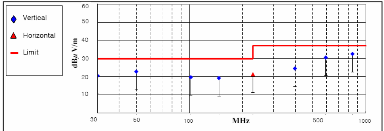
< Fig 9. Radiated emission result (30 MHz ~ 1 000 MHz)>
