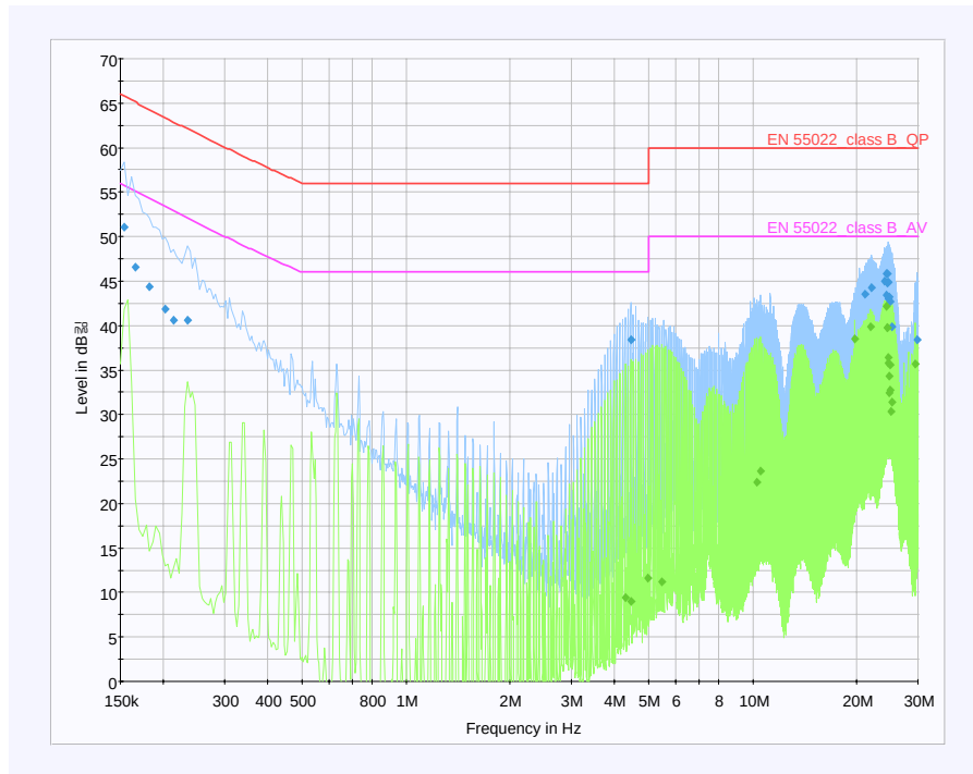
< Live line >
